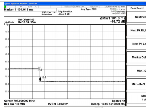
Lower 700MHz band Variable Uplink Noise Timing
