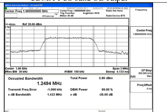
CDMA-PCS band DL output
