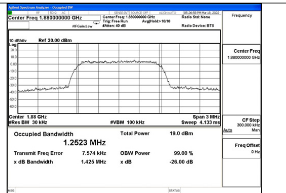
CDMA-PCS band UL output
