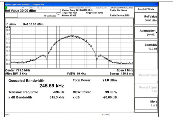
GSM-Upper 700 band UL output
