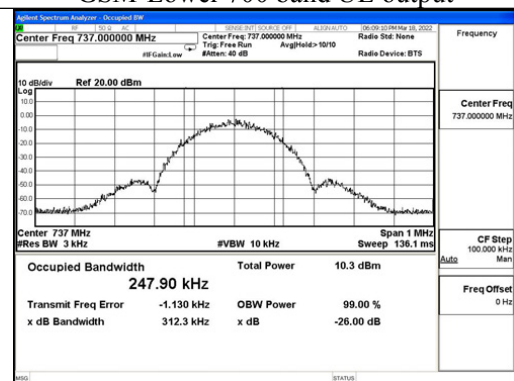
GSM-Lower 700 band DL output
