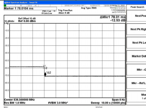
Cellular band Variable Uplink Noise Timing
