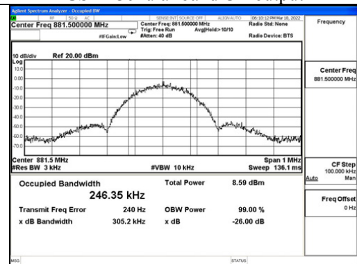
GSM-Cellular band DL output
