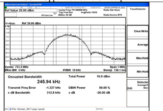
GSM-Upper 700 band DL output
