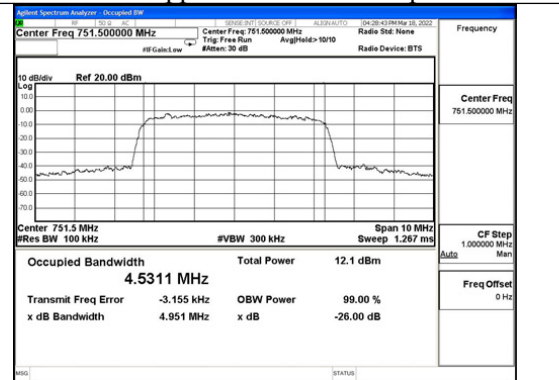
LTE-Upper 700 band DL output
