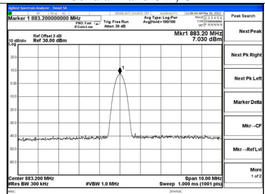
Cellular Band CW, DL
