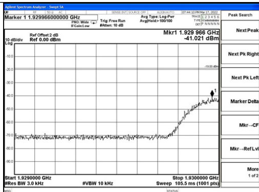
PCS Band GSM DL Left Side Pre AGC
