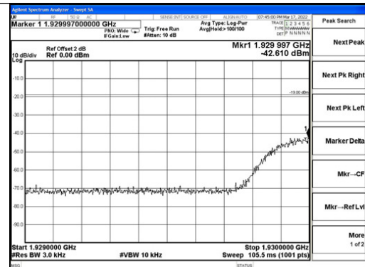
PCS Band GSM DL Left Side 10dB Above AGC
