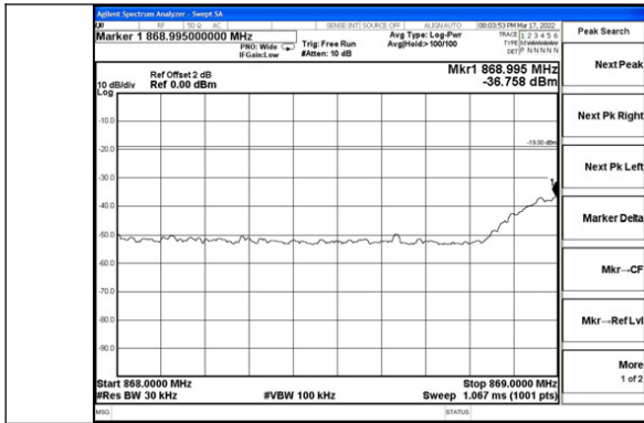
Cellular Band CDMA DL Left Side Pre AGC
