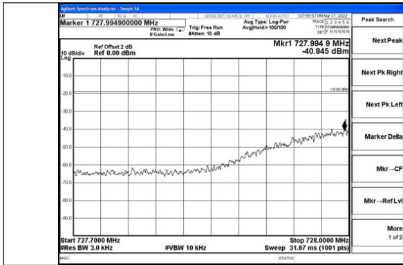
Lower 700MHz band GSM DL Left Side Pre AGC
