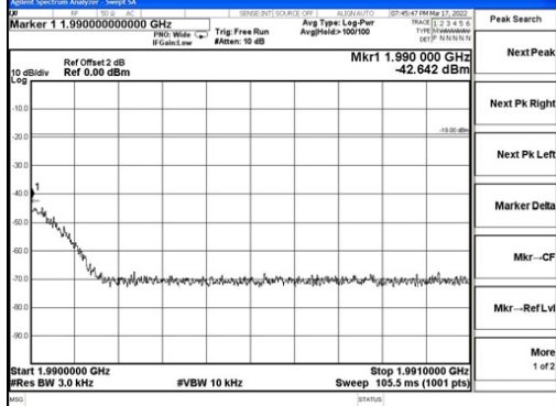
PCS Band GSM DL Right Side Pre AGC
