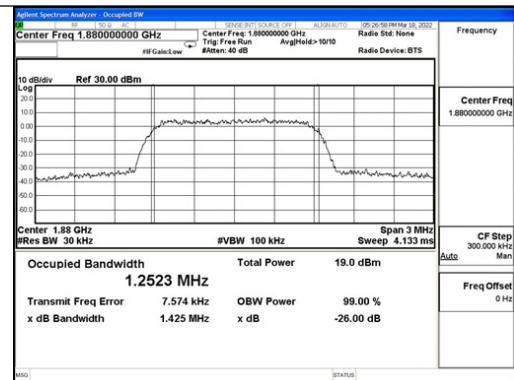
CDMA-PCS band UL output
