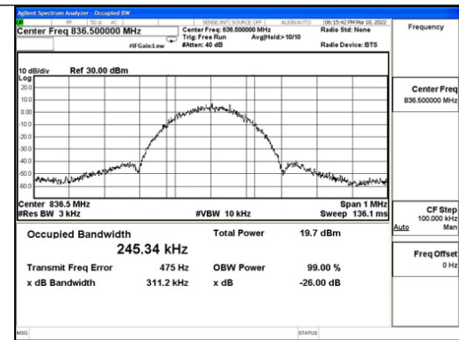
GSM-Cellular band UL output
