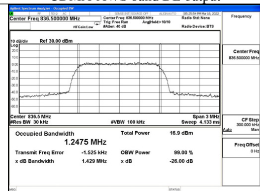
CDMA-Cellular band UL output
