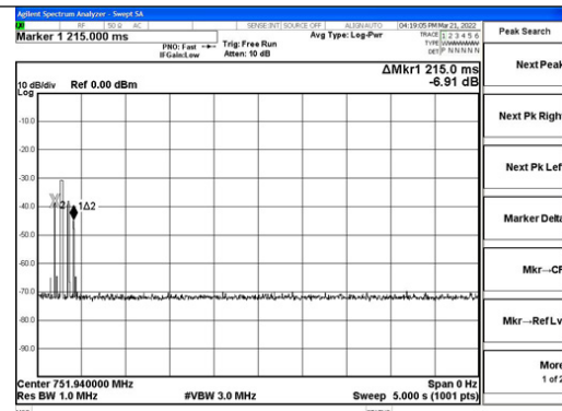
detection time-Upper 700 band DL
