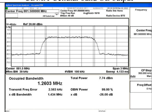
Cellular band DL output
