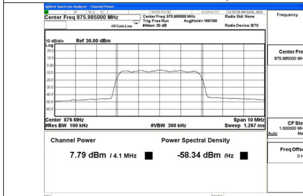
Cellular Band AWGN, DL
