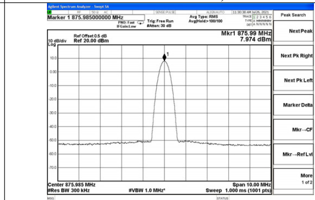
Cellular Band CW, DL
