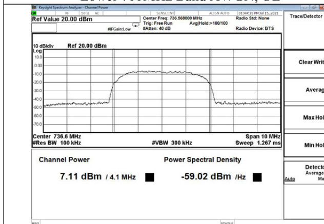
Lower 700MHz Band AWGN, DL
