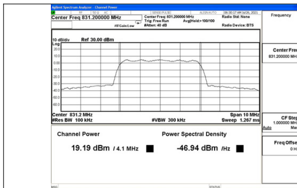
Cellular Band AWGN, UL
