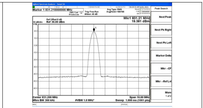
Cellular Band CW, UL
