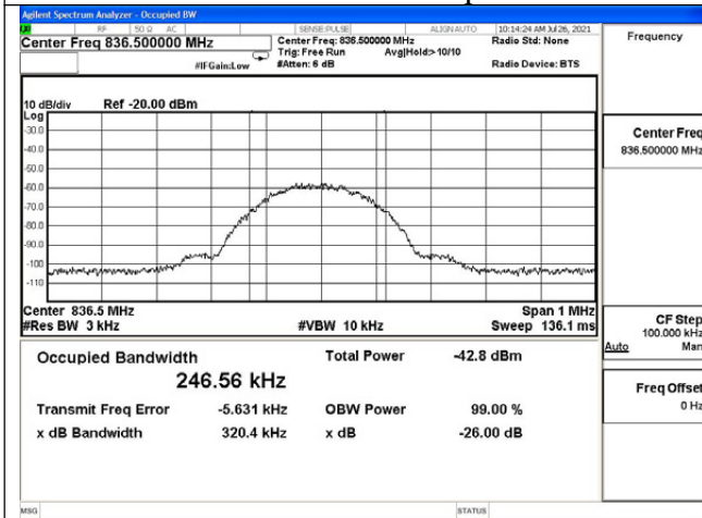
Cellular band UL input
