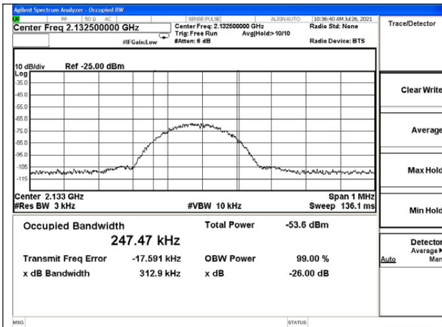
AWS band DL input
