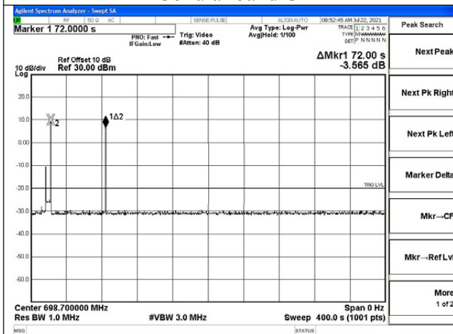
Lower 700 band UL
