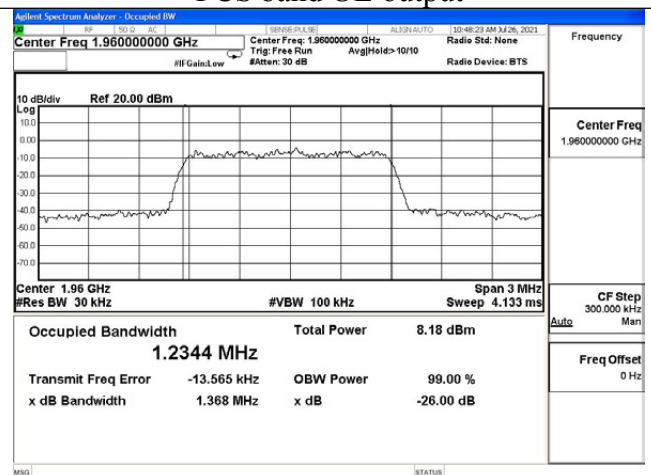
PCS band DL output
