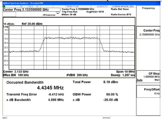
AWS band DL output
