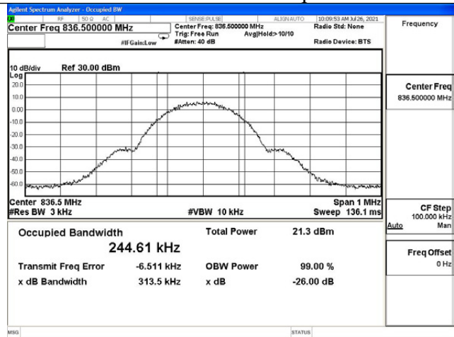
Cellular band UL output
