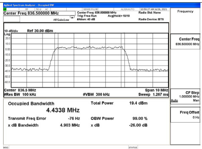
Cellular band UL output
