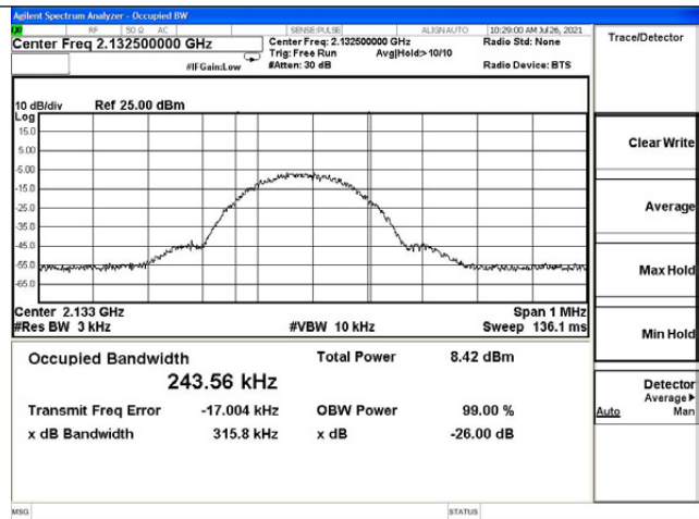
AWS band DL output
