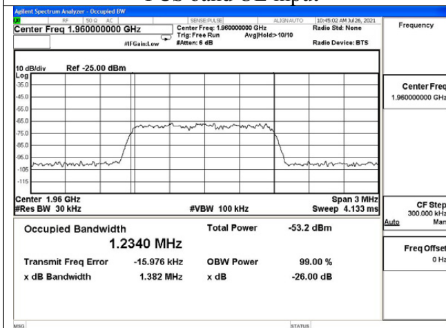
PCS band DL input
