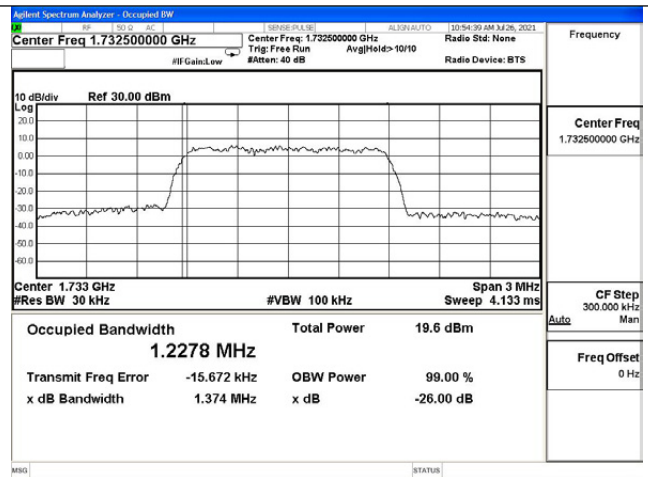
AWS band UL output
