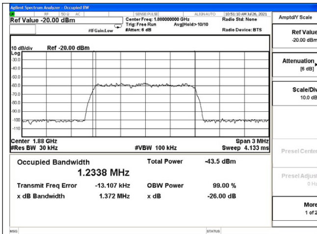
PCS band UL input
