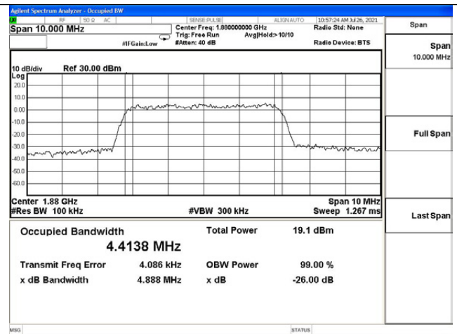
PCS band UL output
