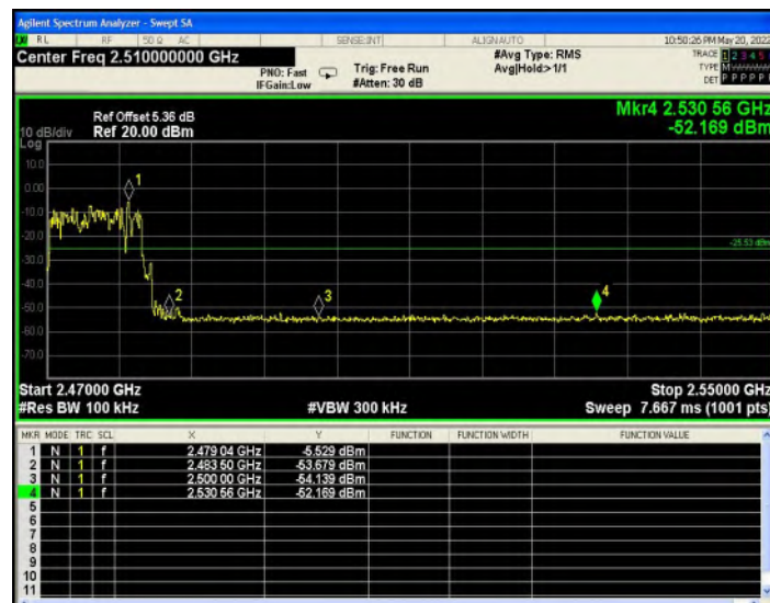
2DH5_Ant1_High_Hop_2480
