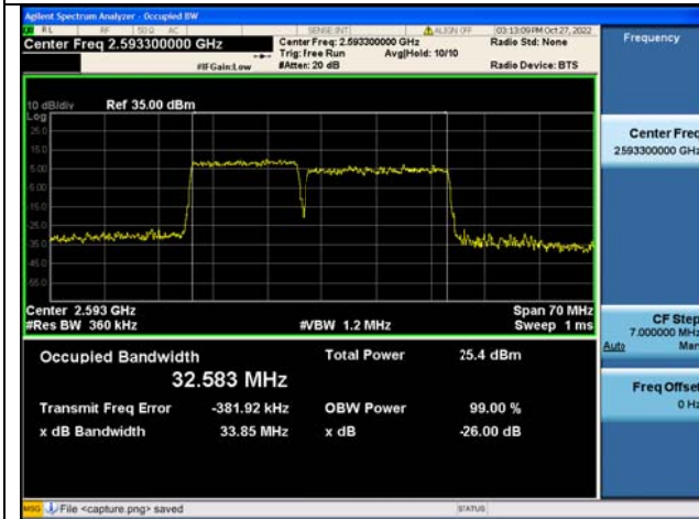
Band41C / 15MHz+20MHz / 16QAM/ Mid CH
