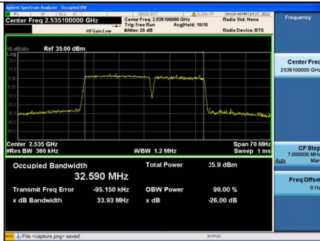
Band7C / 20MHz+15MHz / 64QAM/ Mid CH
