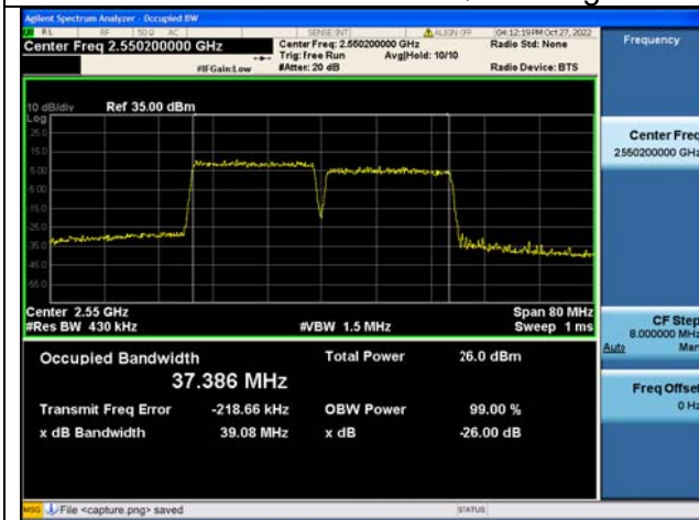
Band7C / 20MHz+20MHz / 64QAM/ High CH
