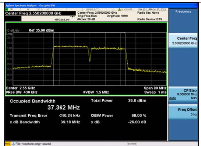
Band7C / 20MHz+20MHz / 16QAM/ High CH
