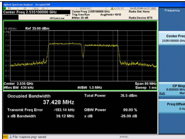
Band7C / 20MHz+20MHz / 16QAM/ Mid CH
