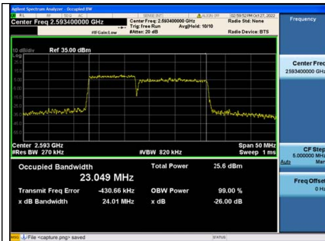
Band41C / 10MHz+15MHz / 64QAM/ Mid CH
