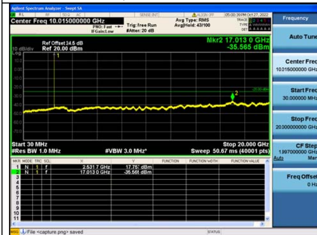
Band7C-30M-20G / 15MHz+20MHz / 1RB+1RB / QPSK / Mid CH
