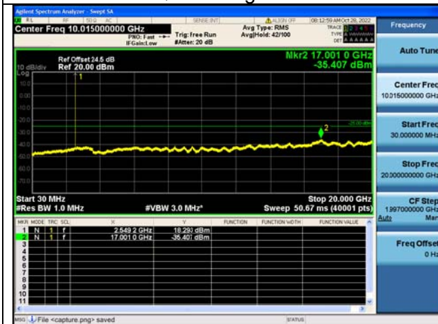
Band7C-30M-20G / 15MHz+20MHz / 1RB+1RB/ QPSK / High CH
