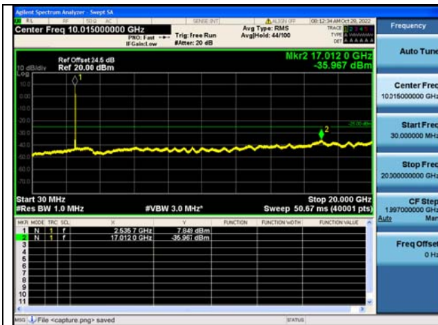
Band7C-30M-20G / 15MHz+20MHz / 1RB+1RB/ QPSK / High CH
