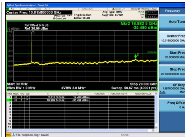
Band7C-30M-20G / 15MHz+20MHz / 1RB+1RB / QPSK / Mid CH
