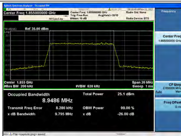
Band25 / 10MHz / 16QAM/ Low CH
