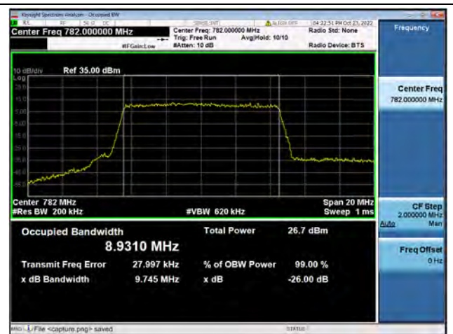
Band13 / 10MHz / 16QAM/ Mid CH
