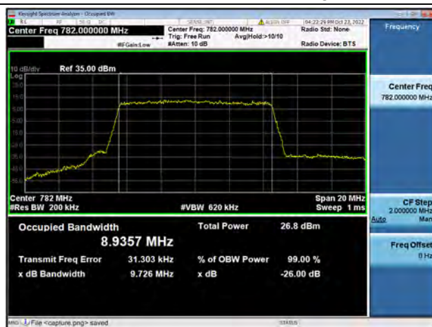
Band13 / 10MHz / 16QAM/ Low CH
