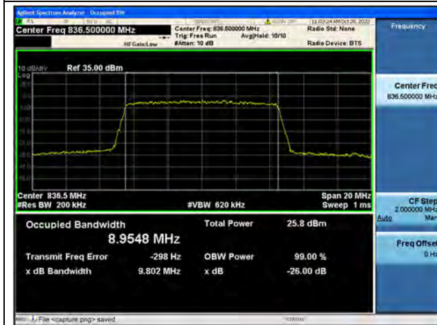
Band5 / 10MHz / 64QAM/ Mid CH
