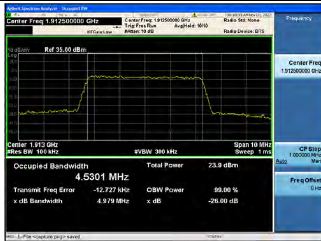
Band25 / 5MHz / 64QAM/ High CH
