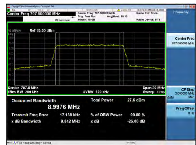
Band12 / 10MHz / QPSK/ Mid CH
