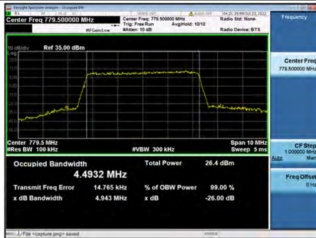
Band13 / 5MHz / 64QAM/ Low CH
