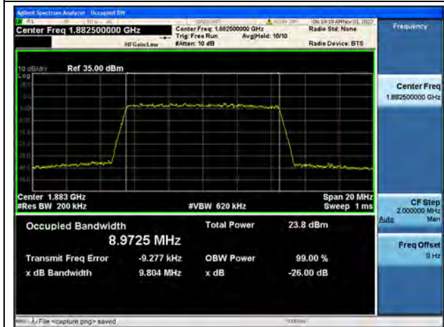
Band25 / 10MHz / 64QAM/ Mid CH
