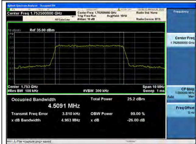
Band4 / 5MHz / 64QAM/ High CH
