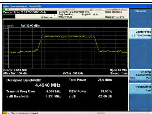
Band38 / 5MHz / 16QAM/ High CH
