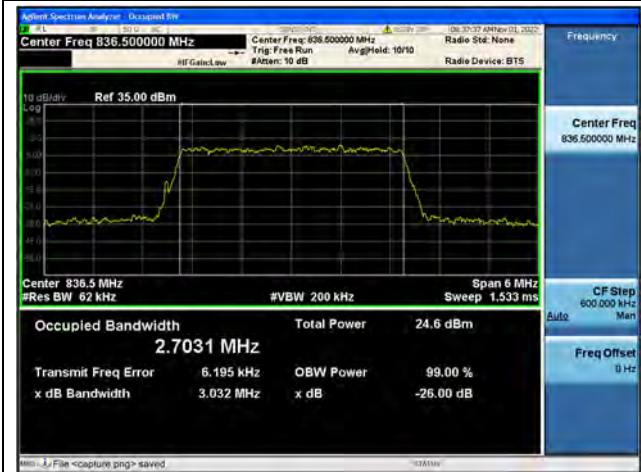
Band26Part22 / 3MHz / 64QAM/ Mid CH
