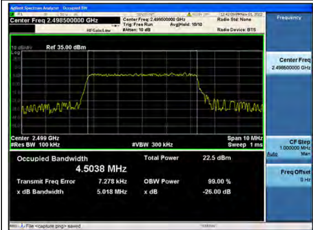
Band41 / 5MHz / 64QAM/ Low CH
