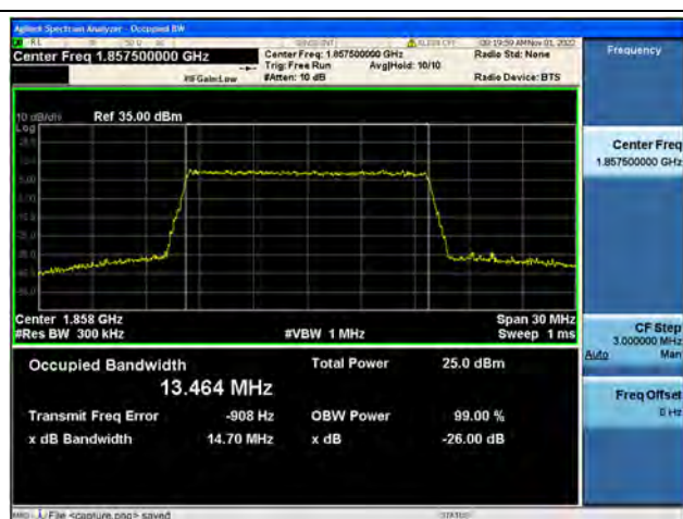
Band25 / 15MHz / 16QAM/ Low CH
