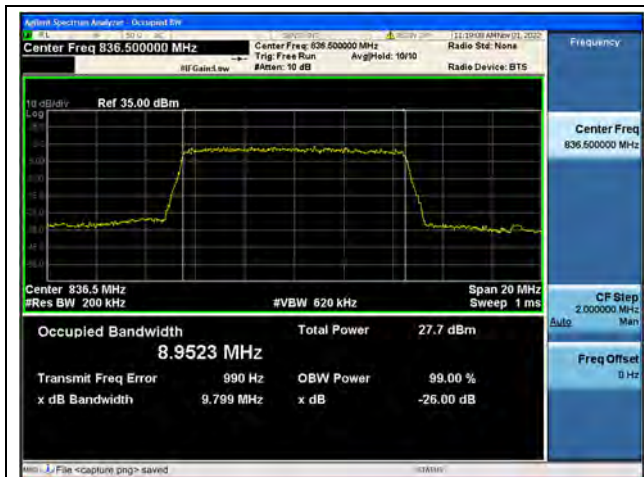
Band26Part22 / 10MHz / QPSK/ Mid CH
