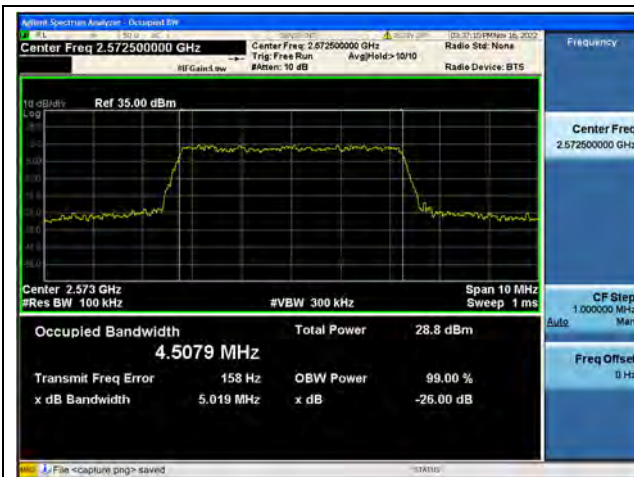
Band38 / 5MHz / QPSK/ Low CH
