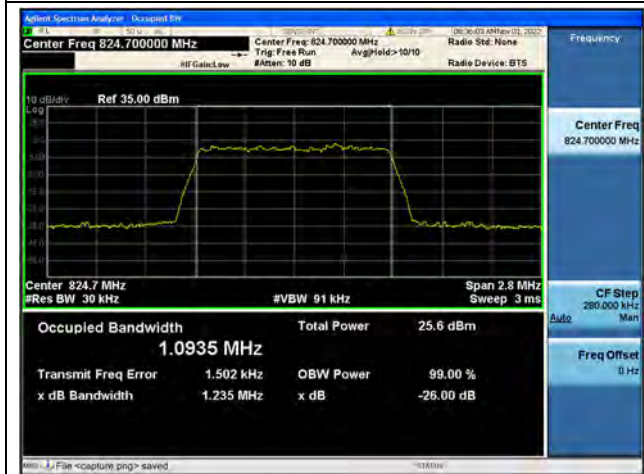
Band26Part22 / 1.4MHz / 64QAM/ Low CH
