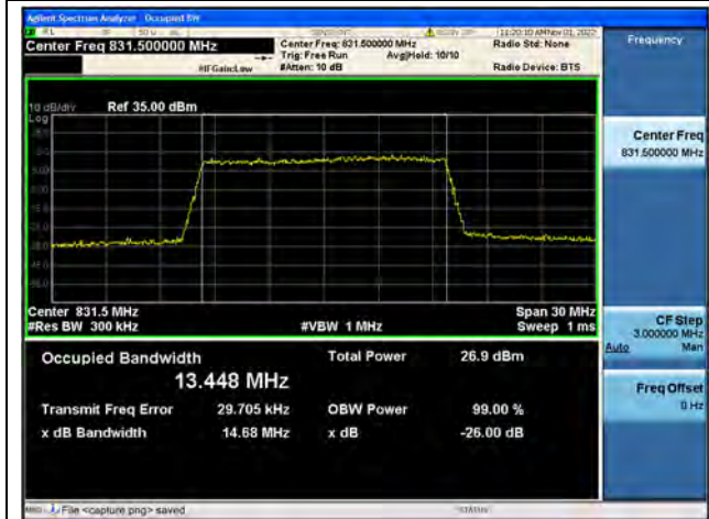
Band26Part22 / 15MHz / 64QAM/ Low CH
