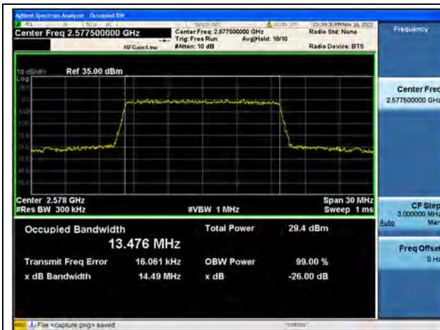
Band38 / 15MHz / QPSK/ Low CH
