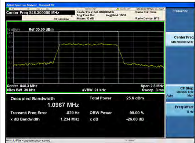
Band26Part22 / 1.4MHz / 64QAM/ High CH
