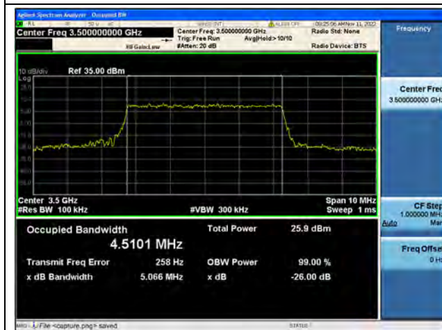
Band42 / 5MHz / 16QAM/ Mid CH
