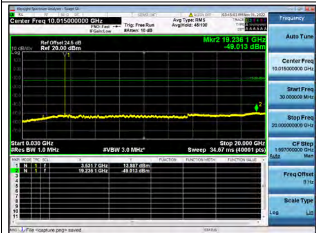
Band42-30M-20G / 20MHz / High CH / 64QAM
