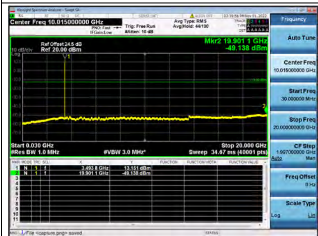
Band42-30M-20G / 15MHz / Mid CH / 64QAM
