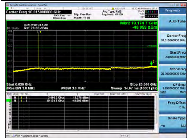
Band42-30M-20G / 10MHz / Mid CH / 16QAM
