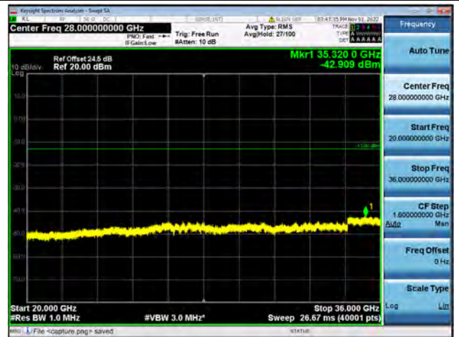
Band42-20G-36G / 20MHz / Mid CH / 16QAM
