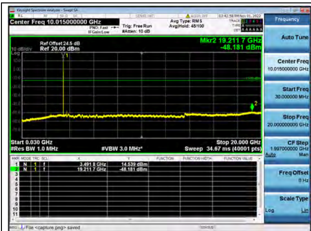
Band42-30M-20G / 20MHz / Mid CH / QPSK
