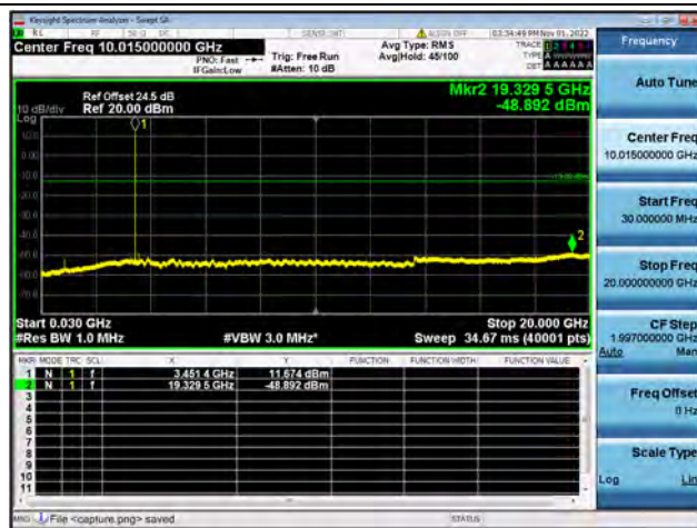
Band42-30M-20G / 10MHz / Low CH / 64QAM
