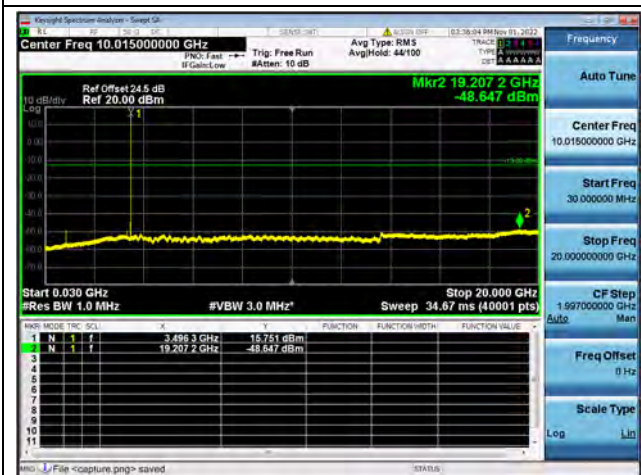
Band42-30M-20G / 10MHz / Mid CH / 64QAM
