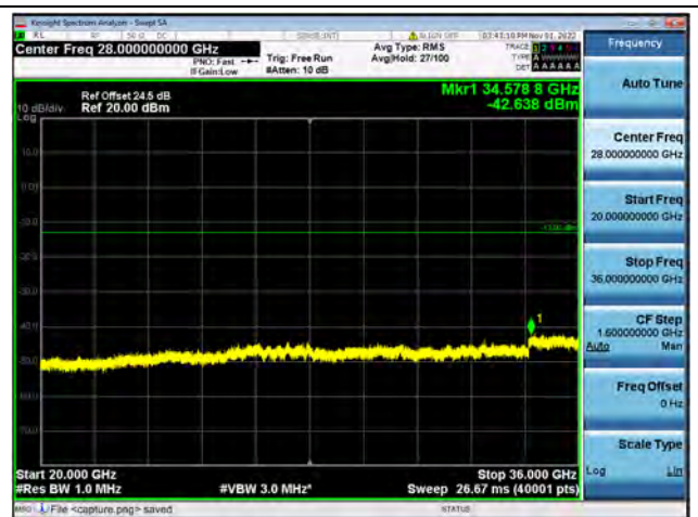
Band42-20G-36G / 20MHz / Mid CH / QPSK
