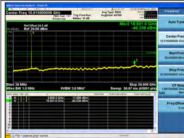
Band41-30M-20G / 15MHz / Mid CH / 16QAM
