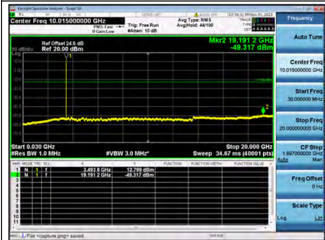
Band42-30M-20G / 15MHz / Mid CH / 16QAM
