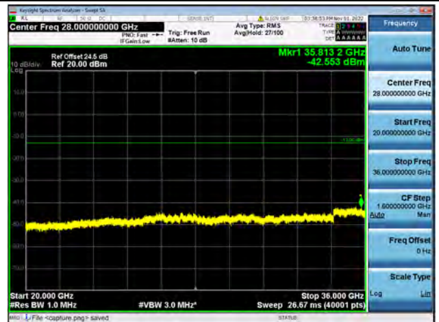
Band42-20G-36G / 15MHz / Low CH / 64QAM
