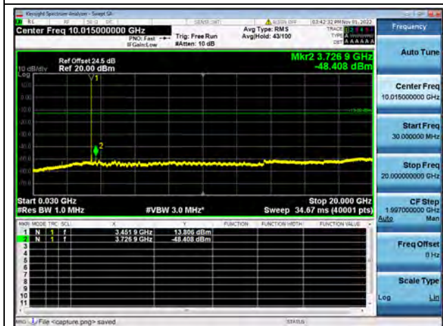
Band42-30M-20G / 20MHz / Low CH / 64QAM
