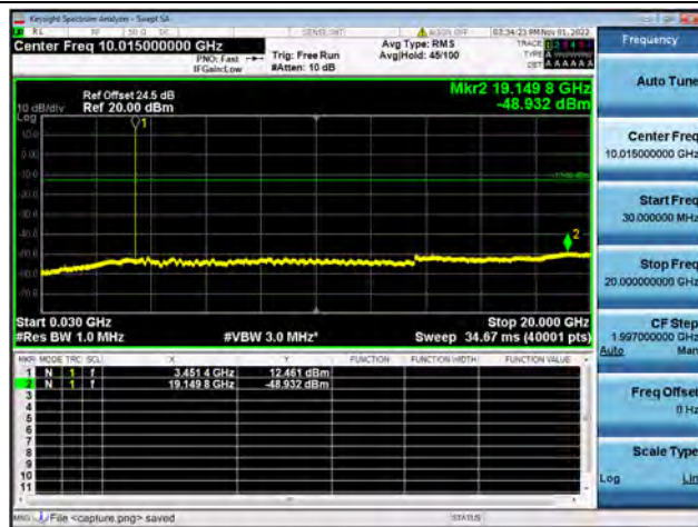
Band42-30M-20G / 10MHz / Low CH / 16QAM
