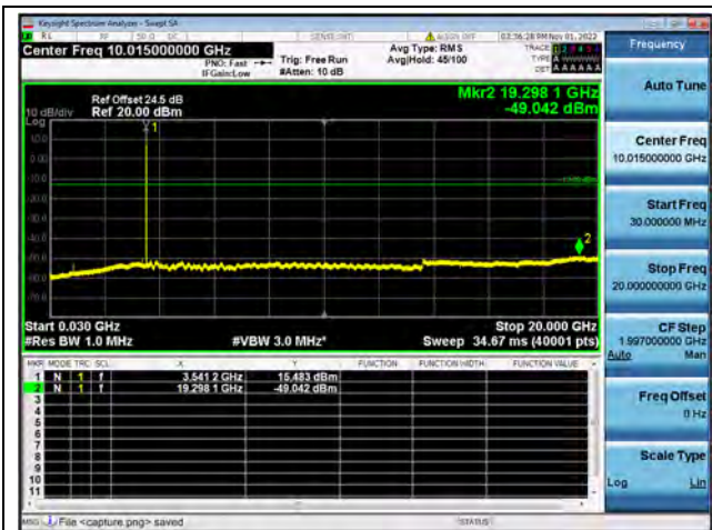
Band42-30M-20G / 10MHz / High CH / QPSK
