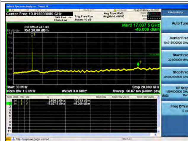
Band41-30M-20G / 15MHz / Mid CH / 64QAM
