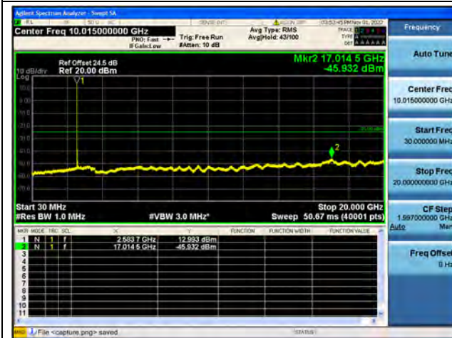
Band41-30M-20G / 20MHz / Mid CH / 16QAM
