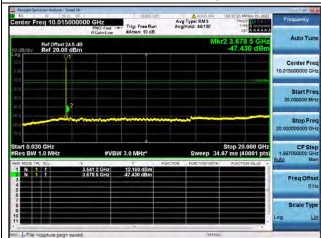
Band42-30M-20G / 10MHz / High CH / 64QAM
