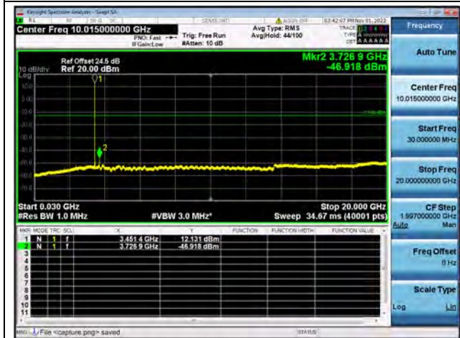
Band42-30M-20G / 20MHz / Low CH / 16QAM
