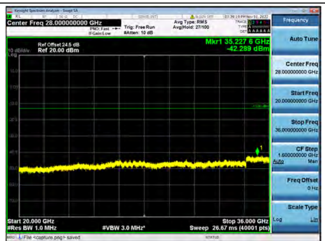
Band42-20G-36G / 15MHz / Mid CH / QPSK
