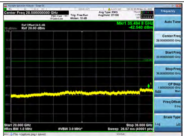
Band42-20G-36G / 5MHz / Mid CH / 64QAM
