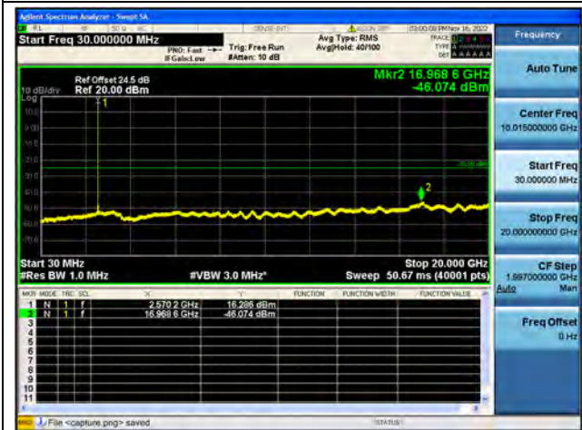
Band38-30M-20G / 5MHz / Low CH / 16QAM
