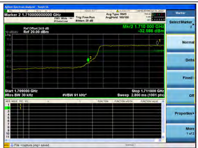
Band66 / 3MHz / Low CH / QPSK / FULL RB
