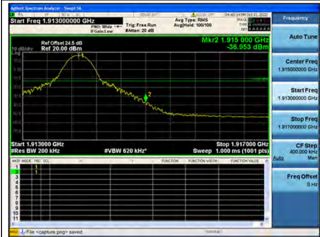
Band25 / 20MHz / High CH / QPSK / 1 RB
