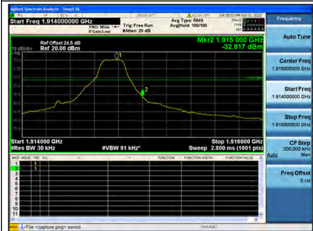
Band25 / 1.4MHz / High CH / QPSK / 1 RB
