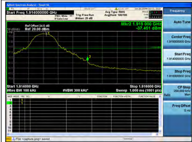
Band25 / 10MHz / High CH / QPSK / 1 RB
