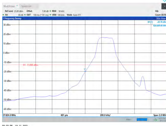
Band26-1.4MHz-QPSK-26797-6RB#0
