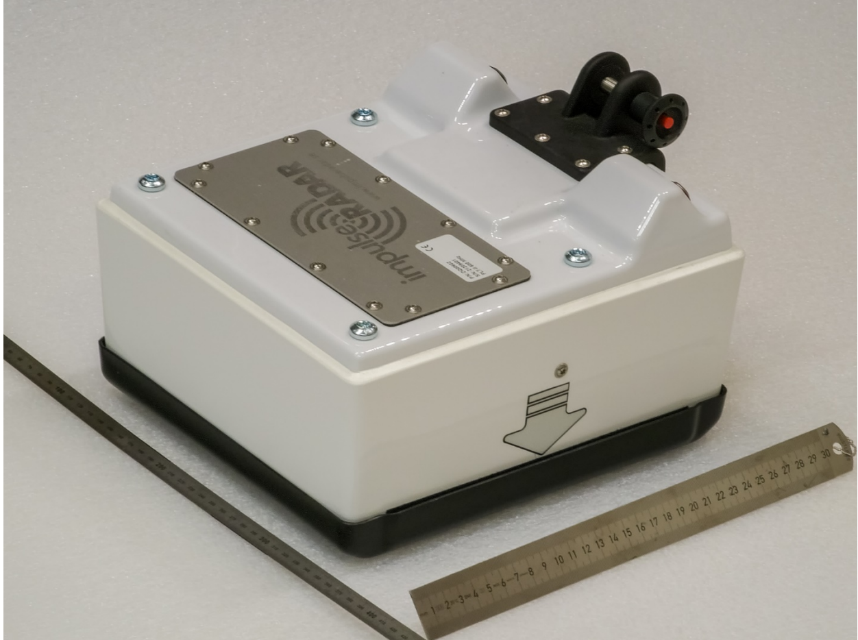
PLT600 Front Side View
