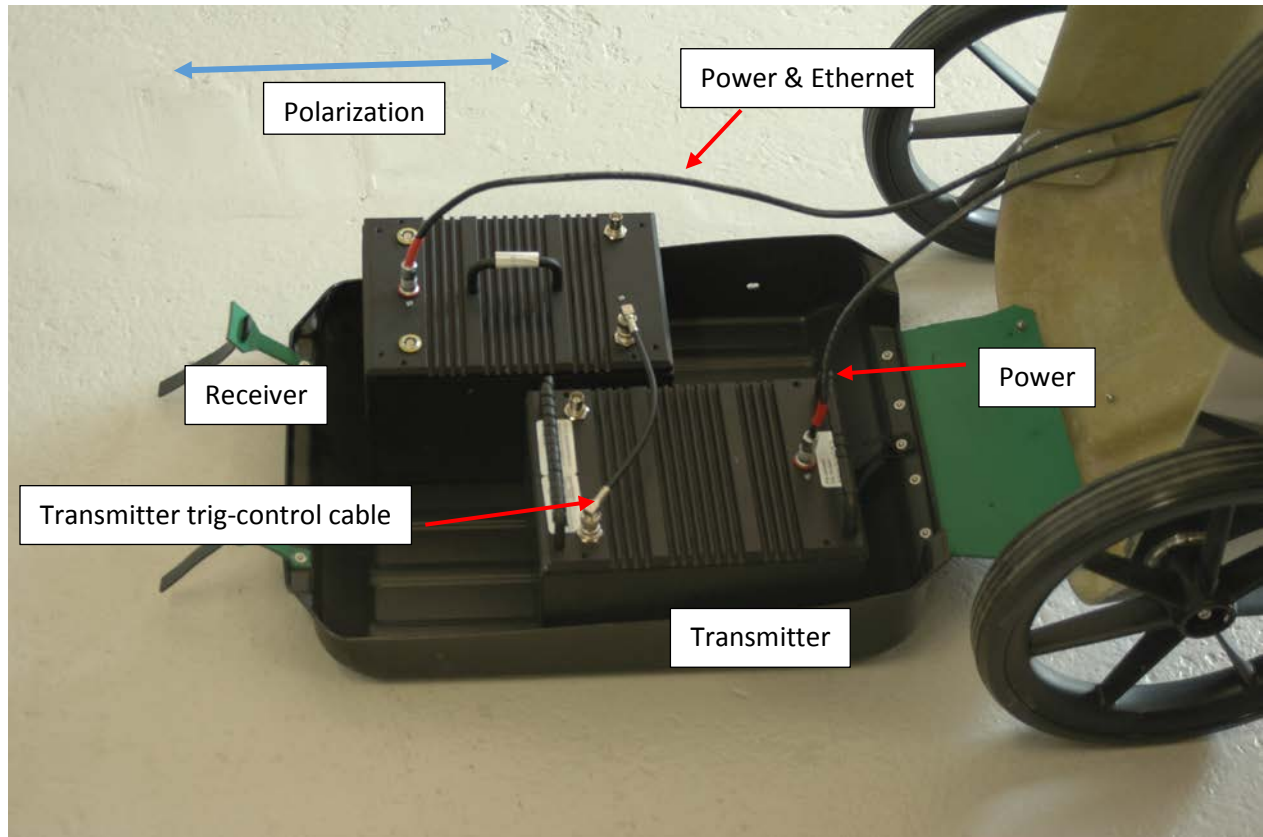
Example configuration, Antennas placed on wear-plate directed towards ground. In-line mounting.
