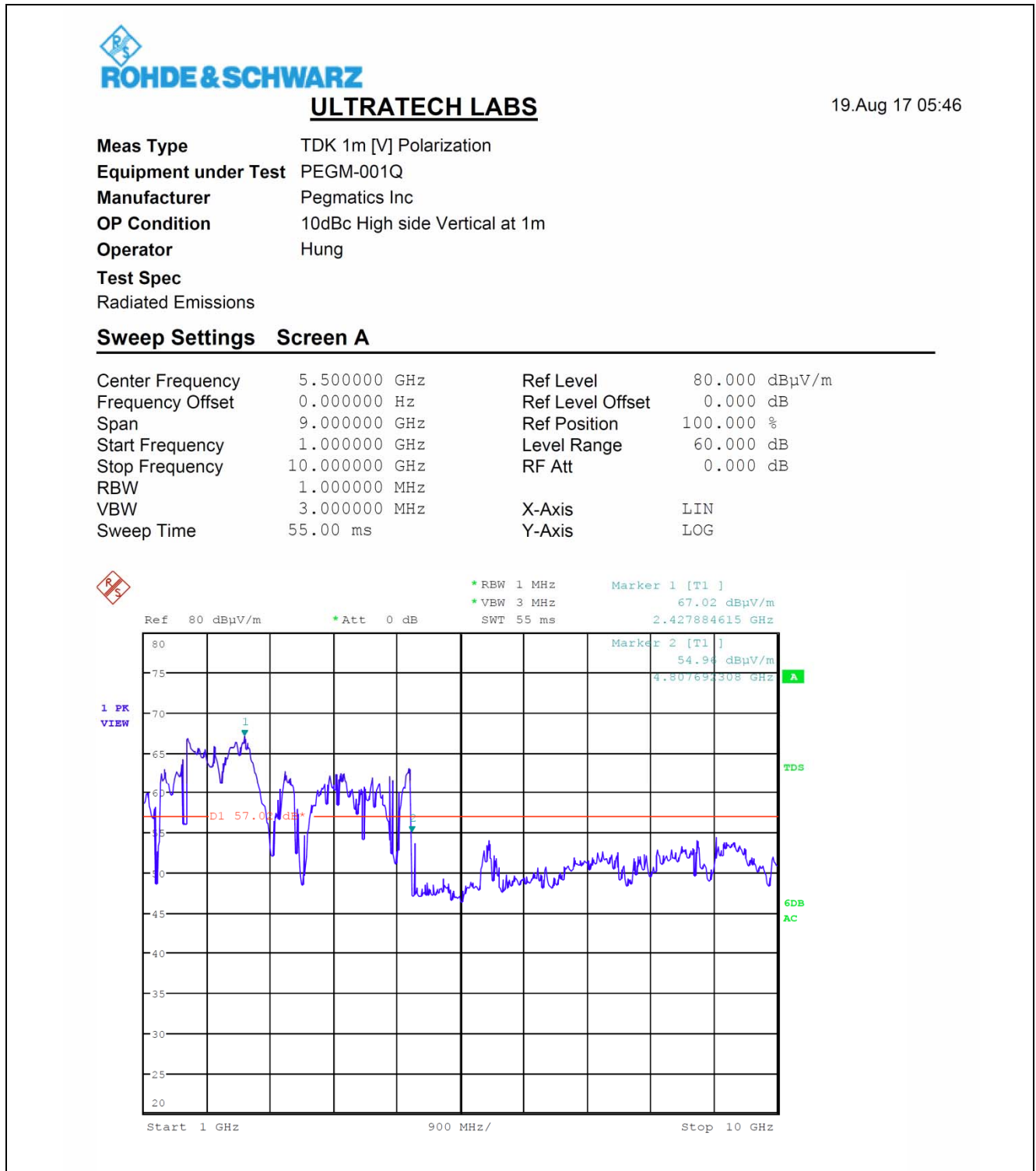
Plot 5.2.3.1. 10 dB Bandwidth, Vertical Polarization, f_M (Marker 1) and f_H (Marker 2)
