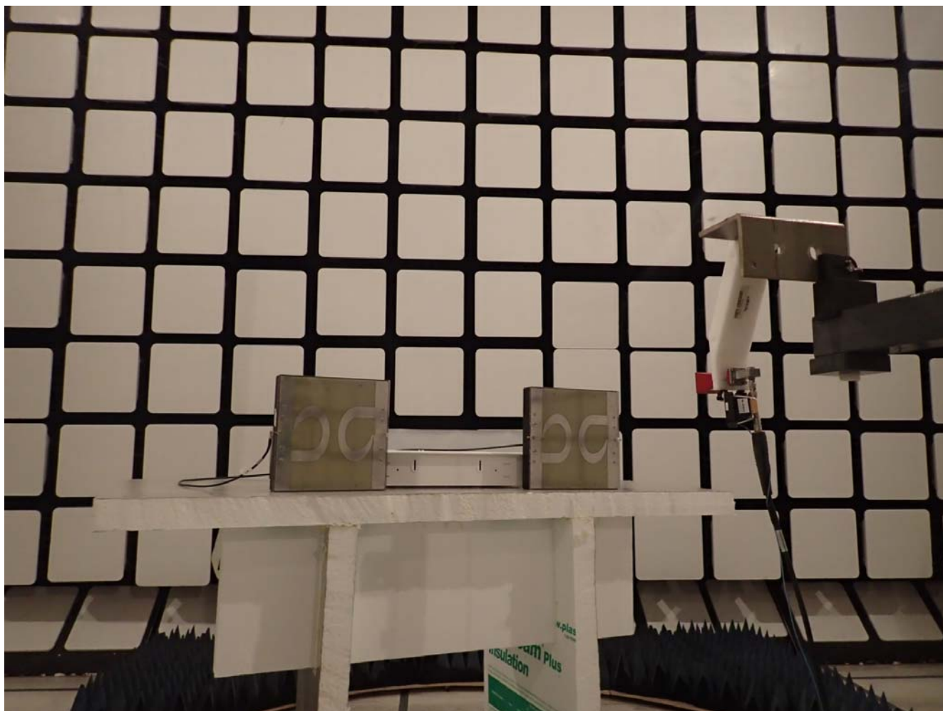
Radiated Emissions at 1 m, Above 1 GHz
