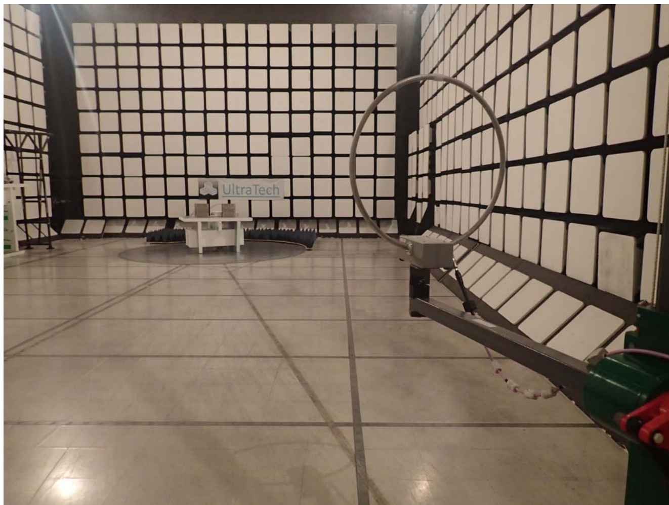
Radiated Emissions at 10 m, 10 kHz to 30 MHz
