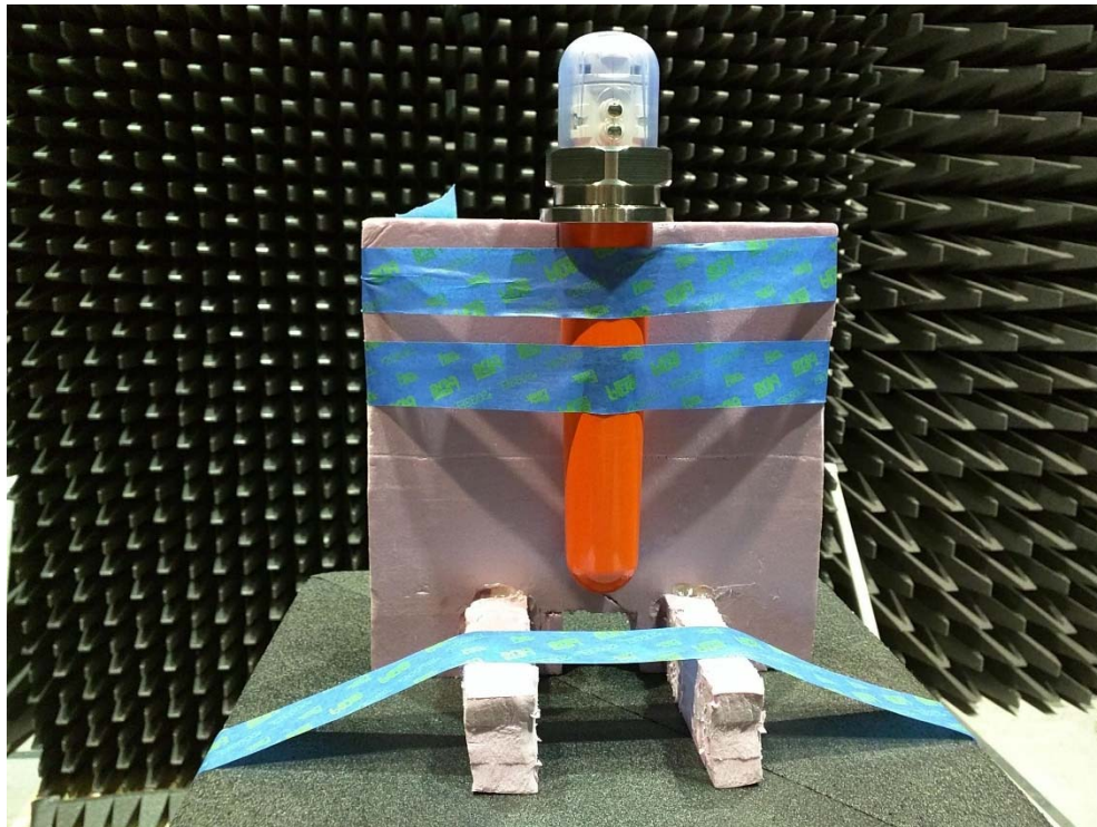
Vertical (Terminals facing antenna)
