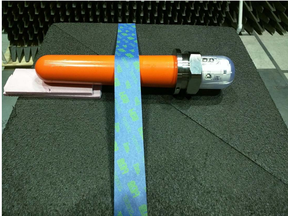
Flat (Terminals up)
