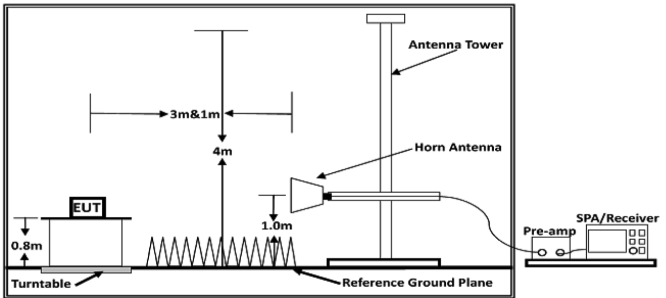
Above 1GHz
