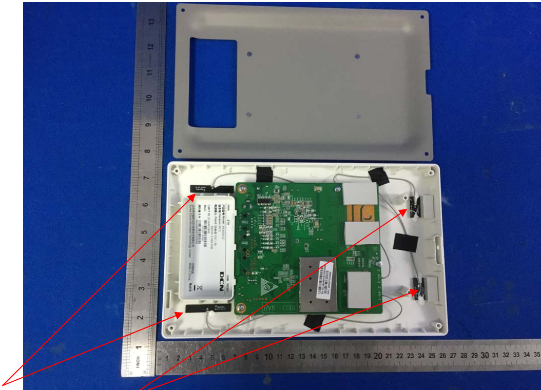
2.4G antenna 5G antenna
