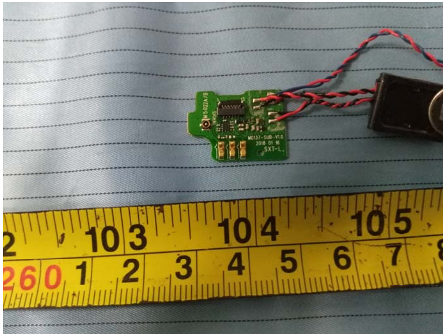
EUT – Small Main Board Top View
