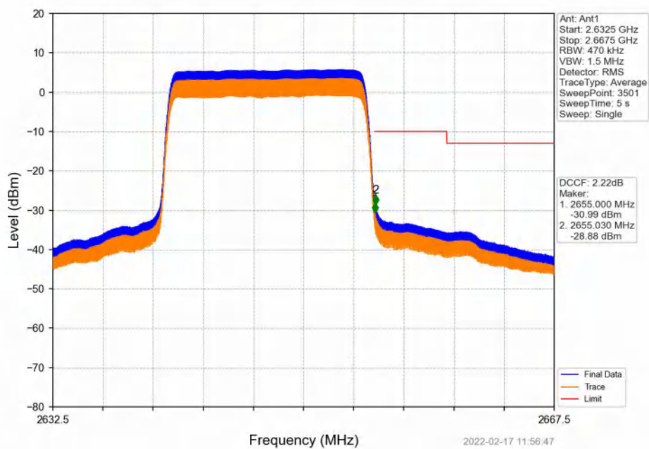
Band41_15MHz_16QAM_HCH_2647.5MHz_RB_75_0_NTNV
