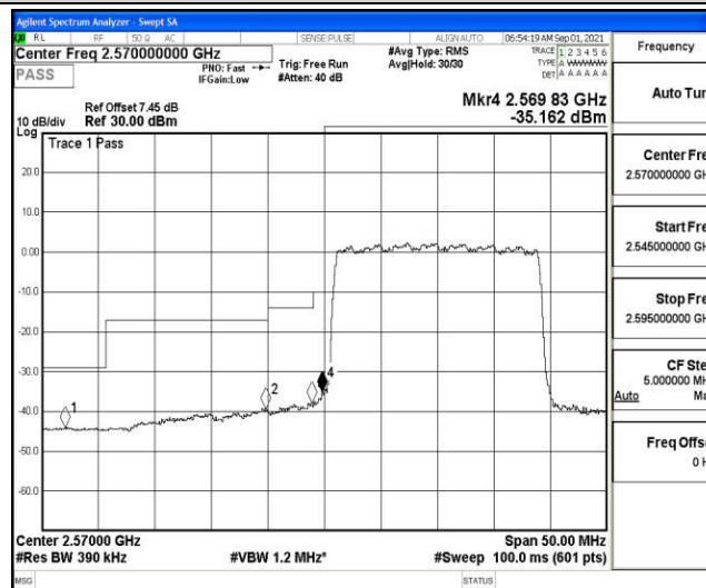
Band38-20MHz-QPSK-38150-100RB#0
