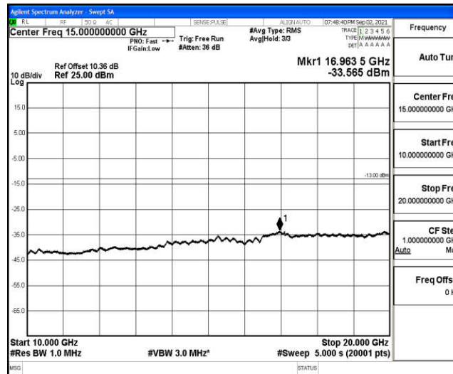
Band66-20MHz-16QAM-132572-1RB#0-Range5:10000~20000MHz
