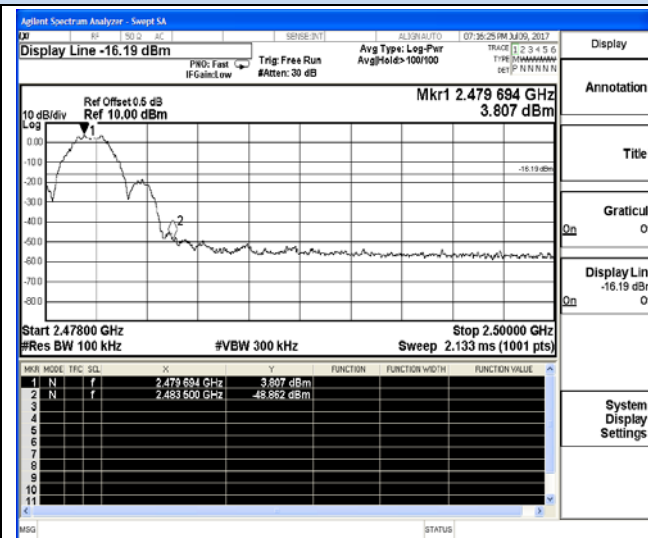
Channel 26 / 2480 MHz
