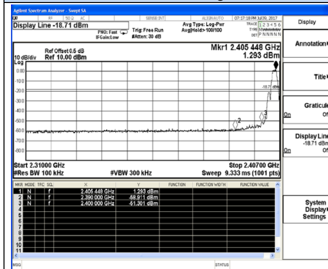
Channel 11 / 2405 MHz
