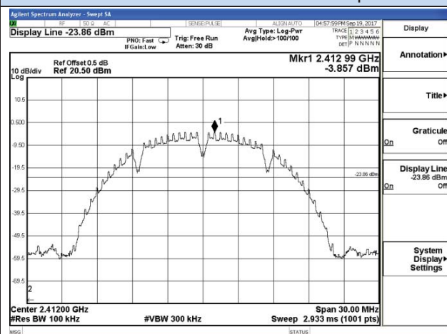
802.11b_Low Channel
