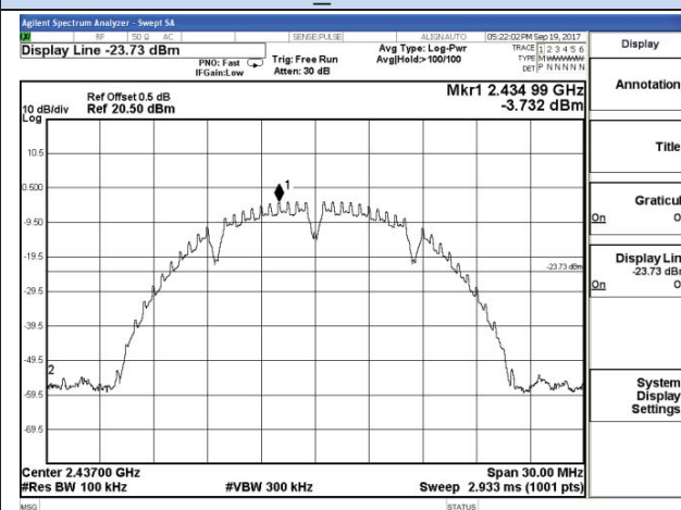
802.11b_Middle Channel
