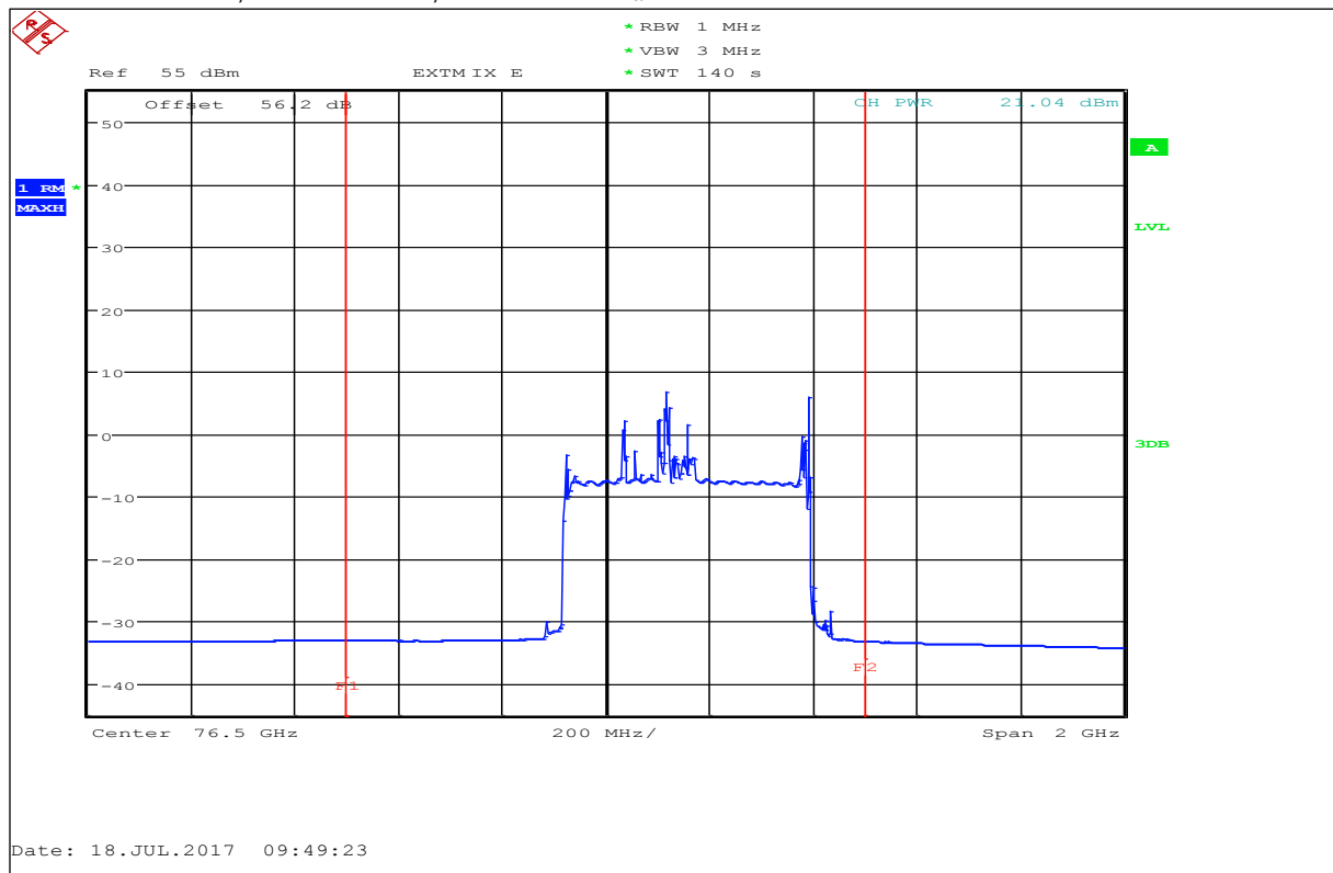
Plot 9: 400 MHz mode, RMS detector, T_{\min} / V_{\min} - V_{\max}
