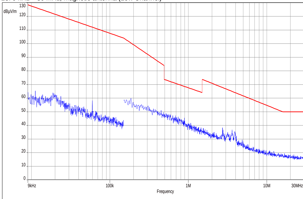
Plot 28: 9 kHz – 30 MHz, Magnetic antenna (Low Channel)
