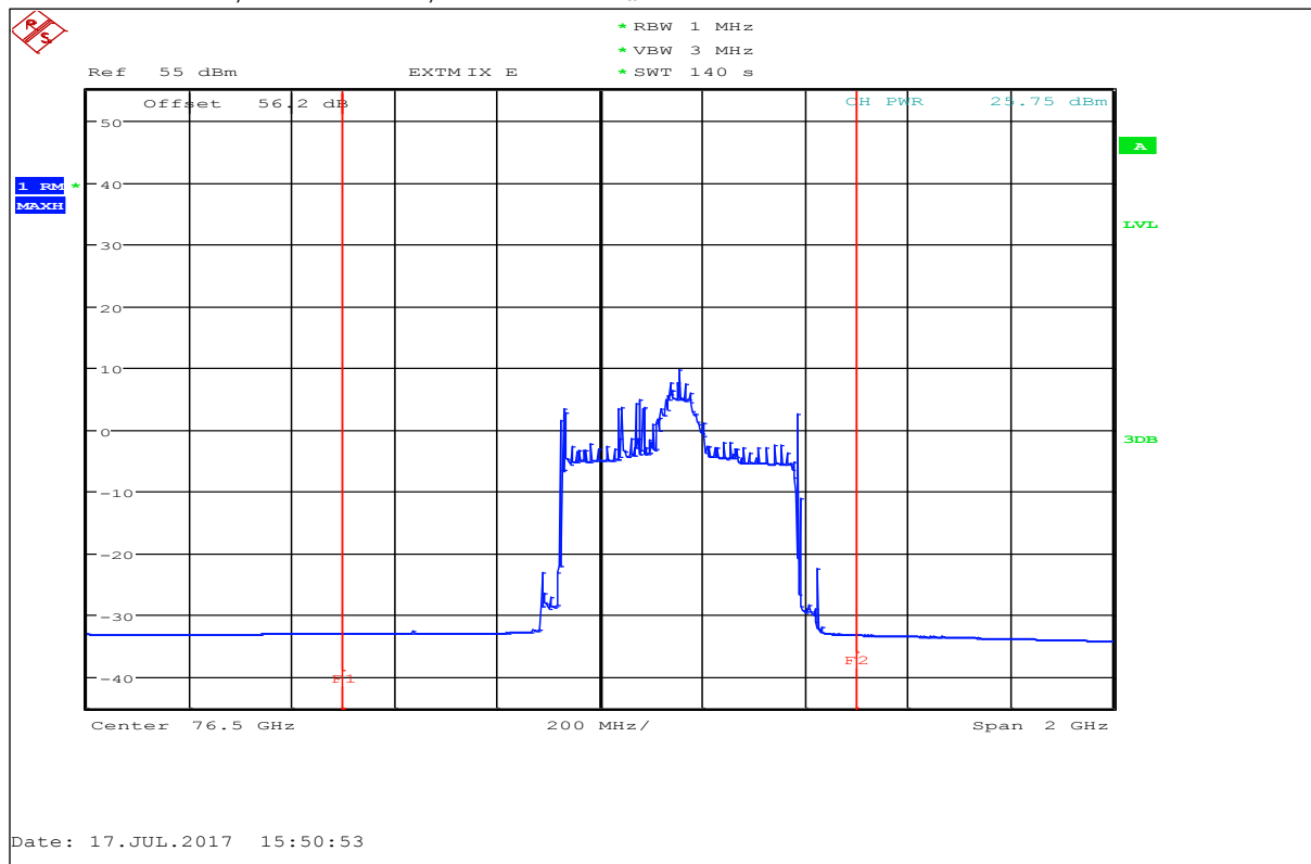
Plot 3: 200 MHz mode, RMS detector, T_{\min} / V_{\min} - V_{\max}
