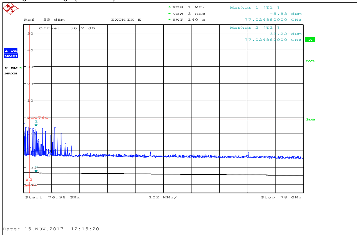
Plot 26: High Band Edge (F>77 GHz)
