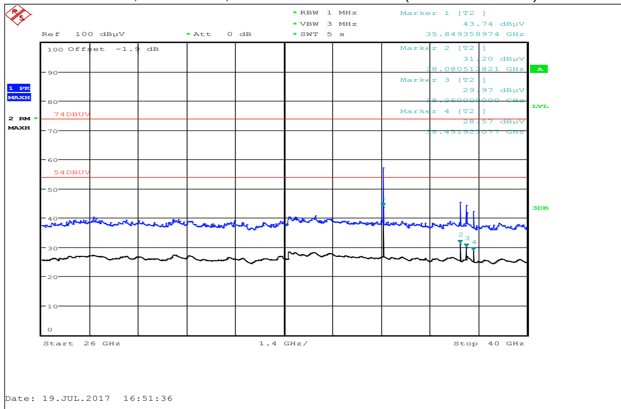
Plot 40: 26 GHz – 40 GHz, RMS detector, antenna vertical / horizontal (valid for all channels)
