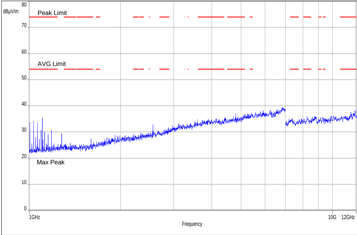
Plot 34: 1 GHz – 12 GHz, antenna vertical / horizontal (Low Channel)
