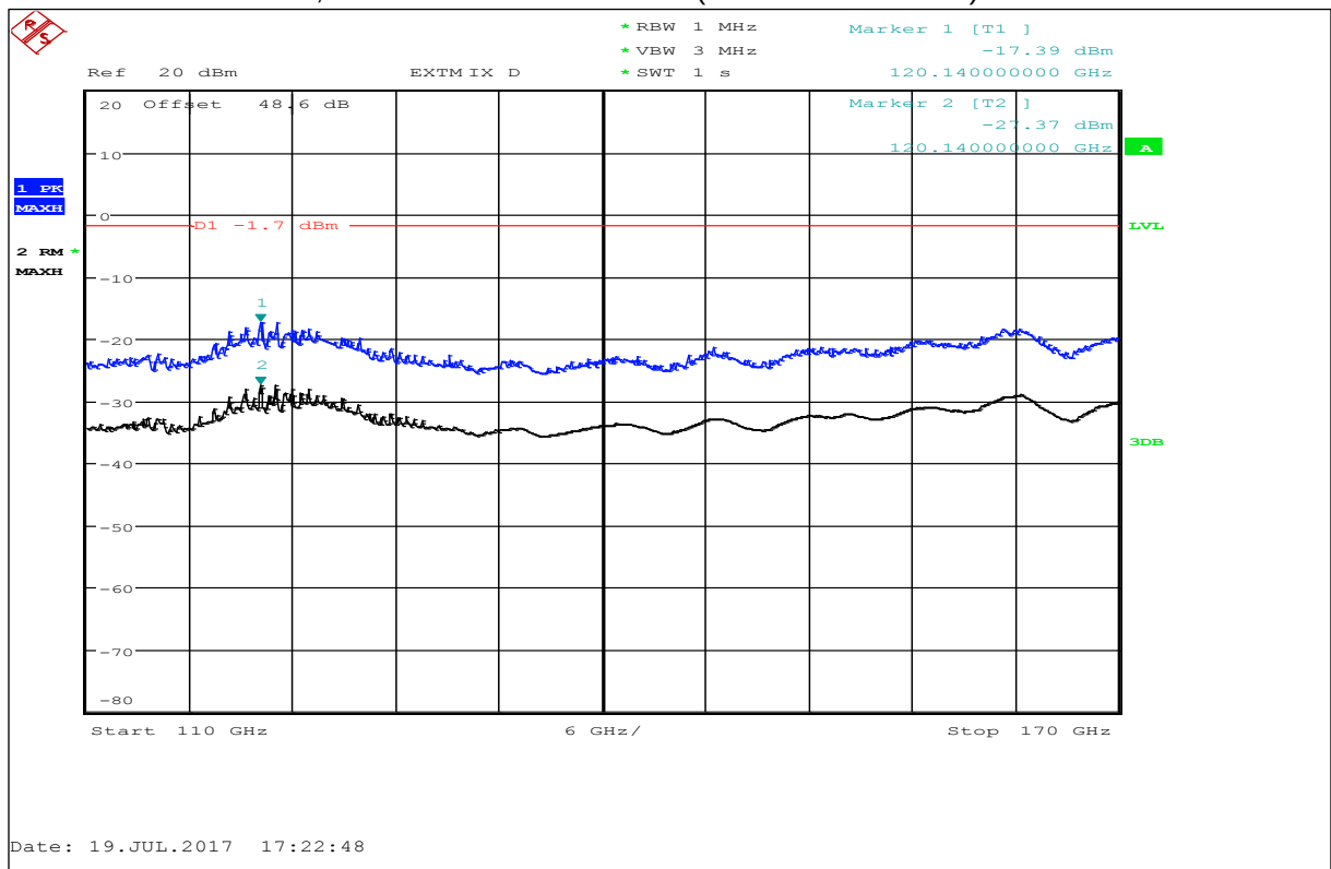
Plot 47: 110 GHz – 170 GHz, antenna vertical / horizontal (valid for all channels)
