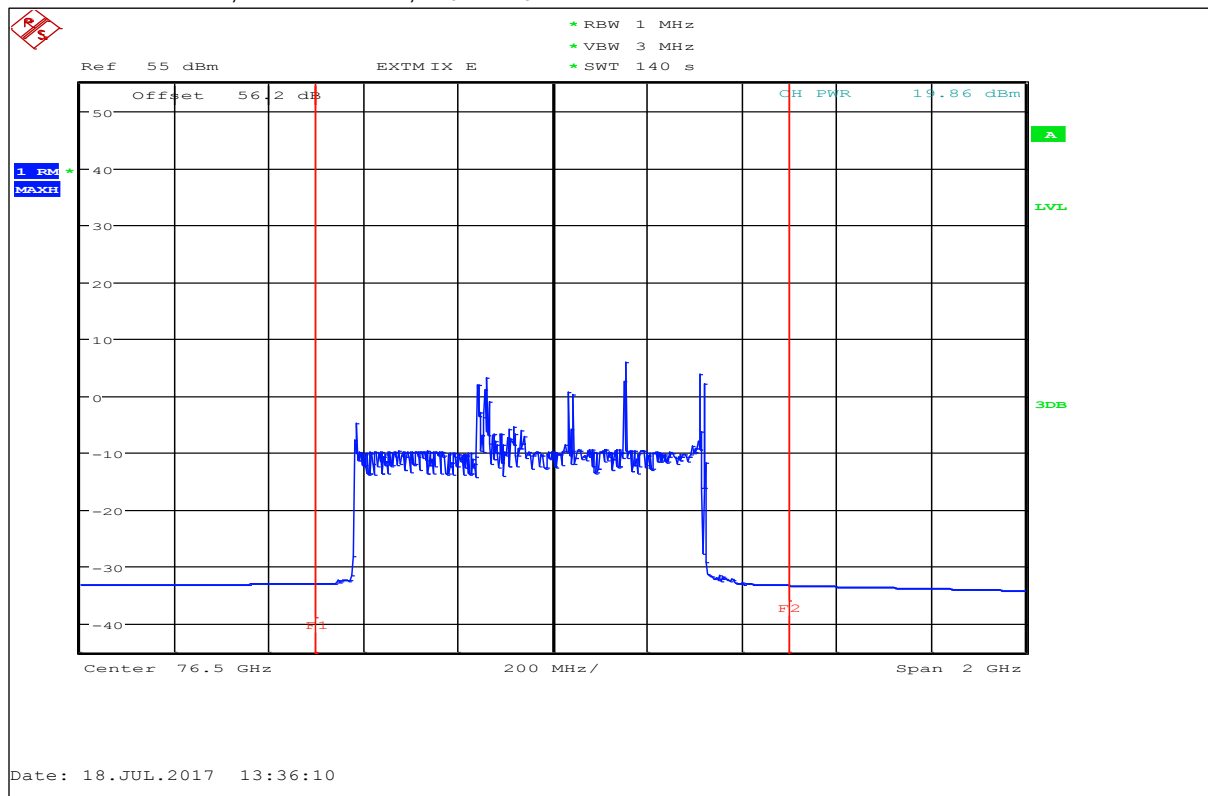
Plot 13: 700 MHz mode, RMS detector, T_{nom} / V_{nom}
