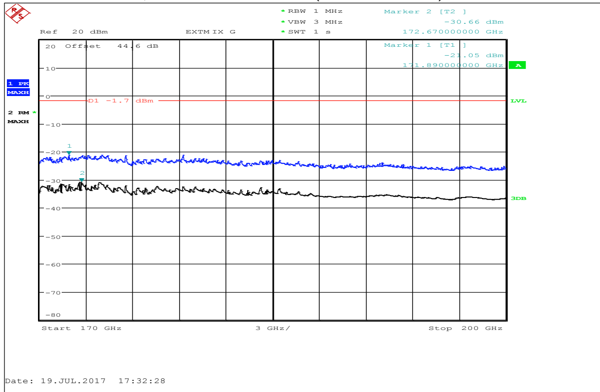
Plot 48: 170 GHz – 200 GHz, antenna vertical / horizontal (valid for all channels)
