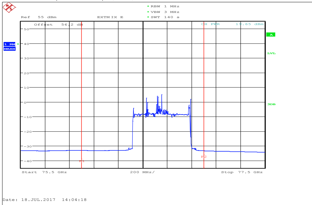
Plot 7: 400 MHz mode, RMS detector, T_{nom} / V_{nom}
