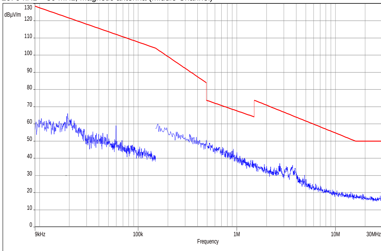
Plot 29: 9 kHz – 30 MHz, Magnetic antenna (Middle Channel)
