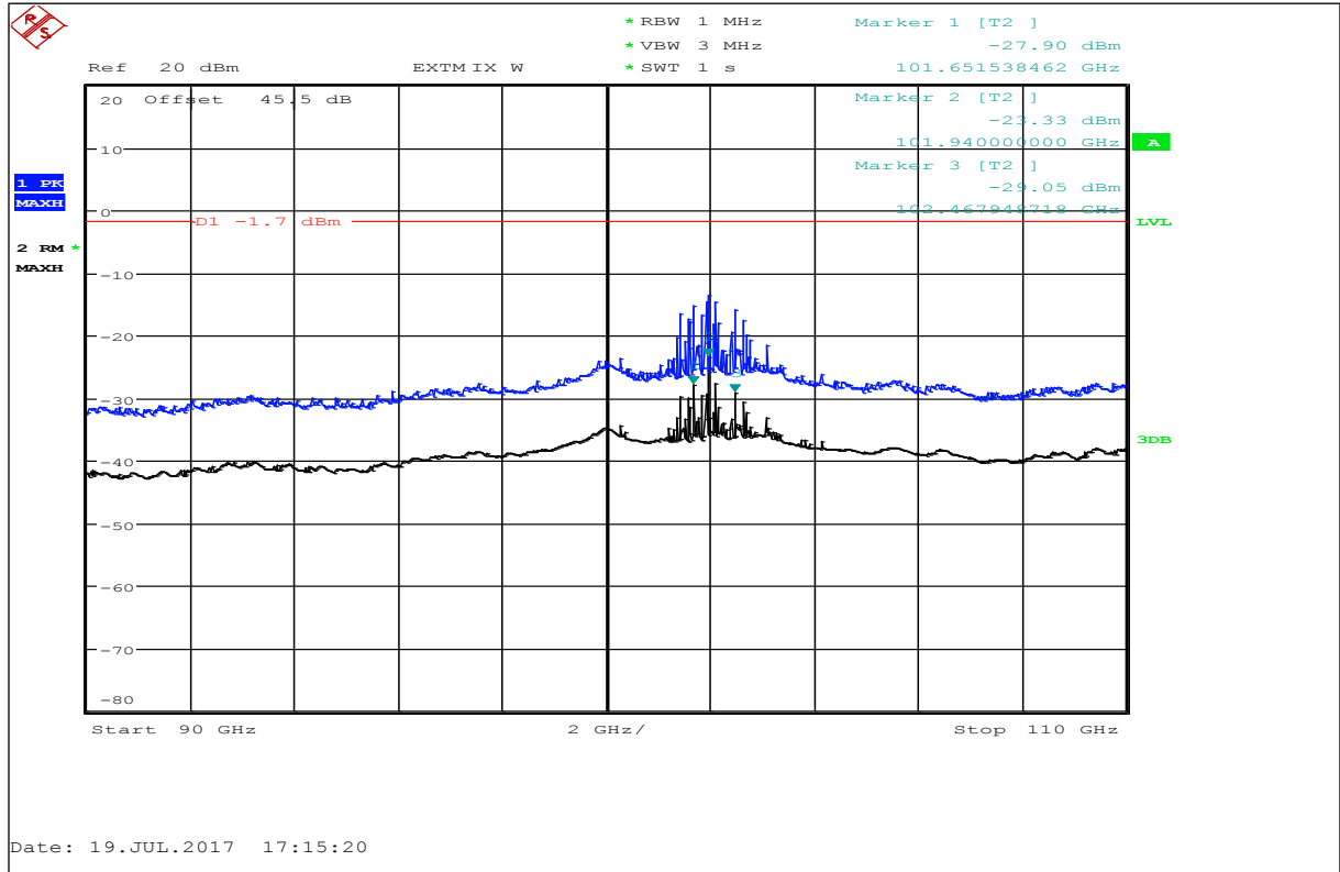
Plot 46: 90 GHz – 110 GHz, RMS detector, antenna vertical / horizontal (valid for all channels)
