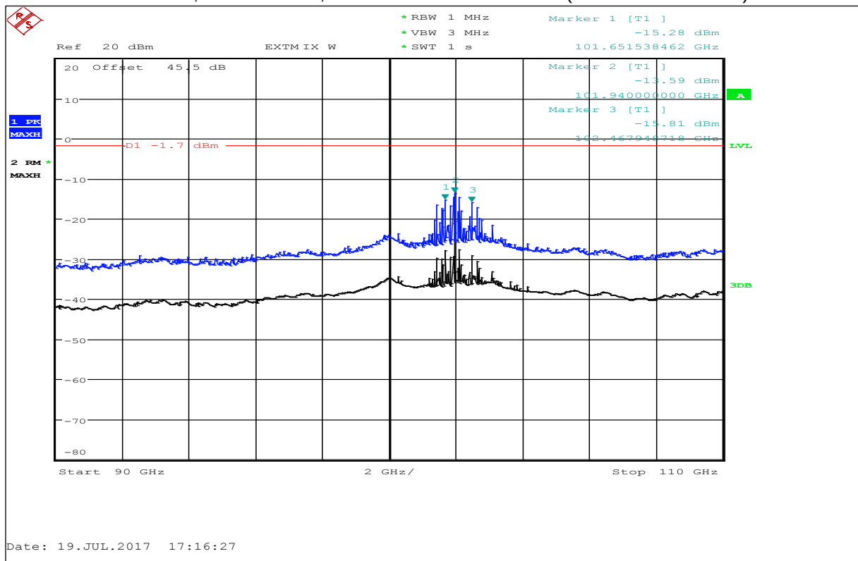
Plot 45: 90 GHz – 110 GHz, Peak detector, antenna vertical / horizontal (valid for all channels)
