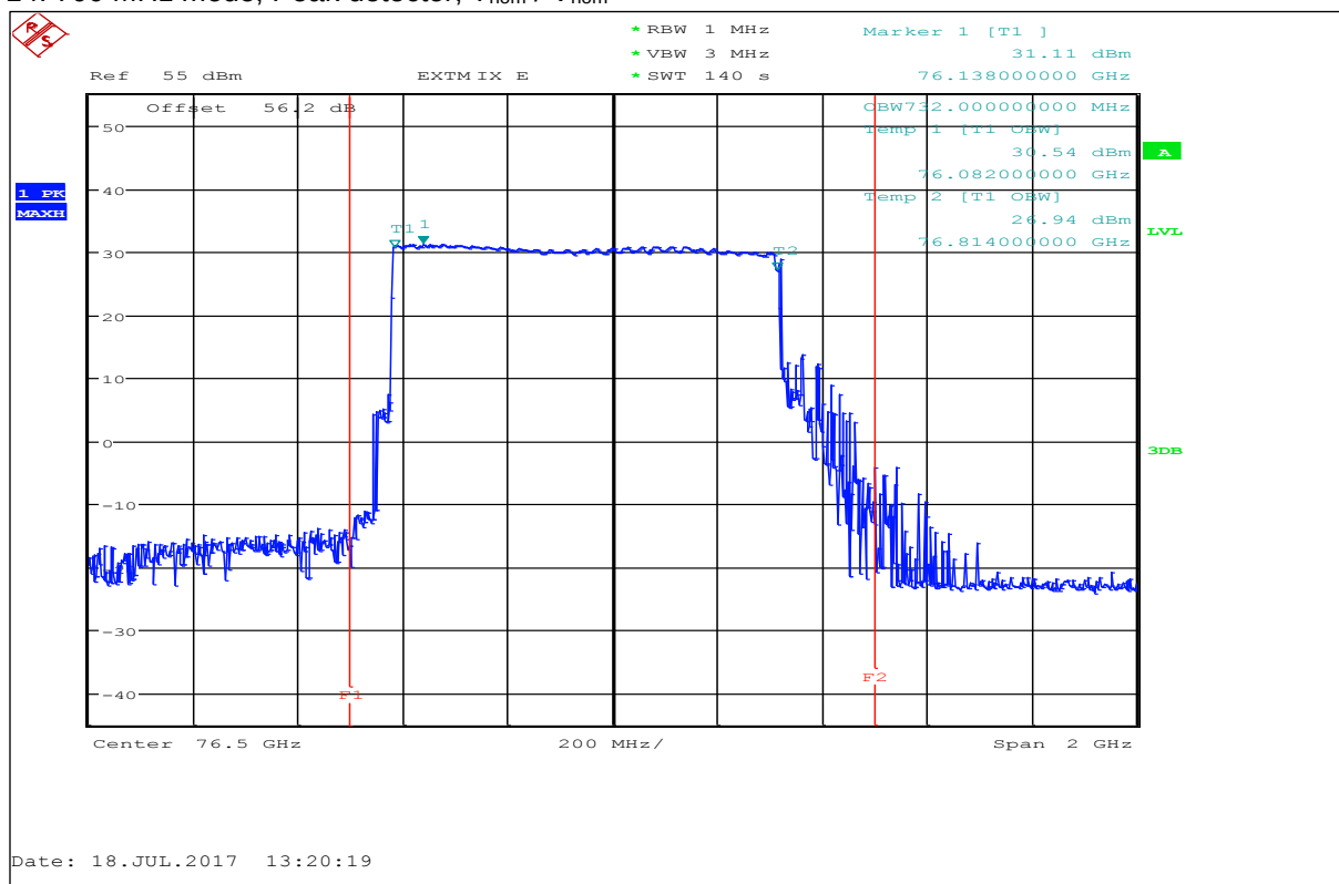
Plot 14: 700 MHz mode, Peak detector, T_{nom} / V_{nom}
