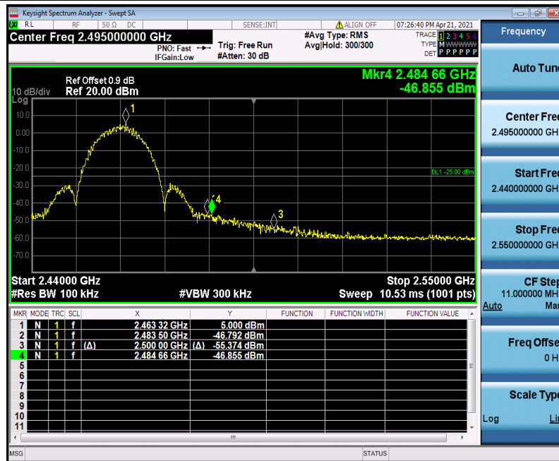
11B_Ant1_High_2462
