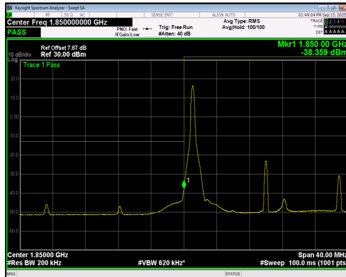
Band2 QPSK BW=20MHz Channel=18700 RB Size=1 Position=#0 Extended
