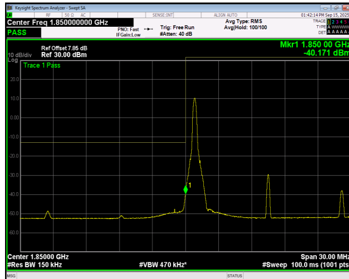
Band2 QPSK BW=15MHz Channel=18675 RB Size=1 Position=#0 Extended
