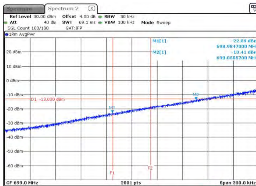
LTE_B12_CH23017_1.4M_QPSK_1RB0_15k
