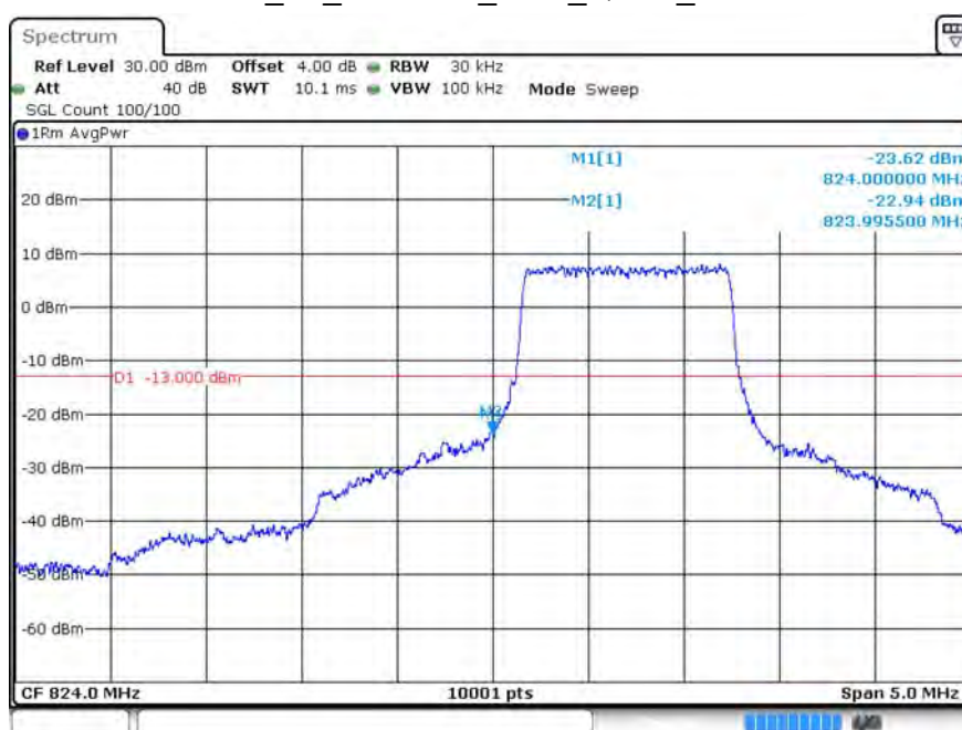
LTE_B5_CH20407_1.4M_QPSK_6RB0
