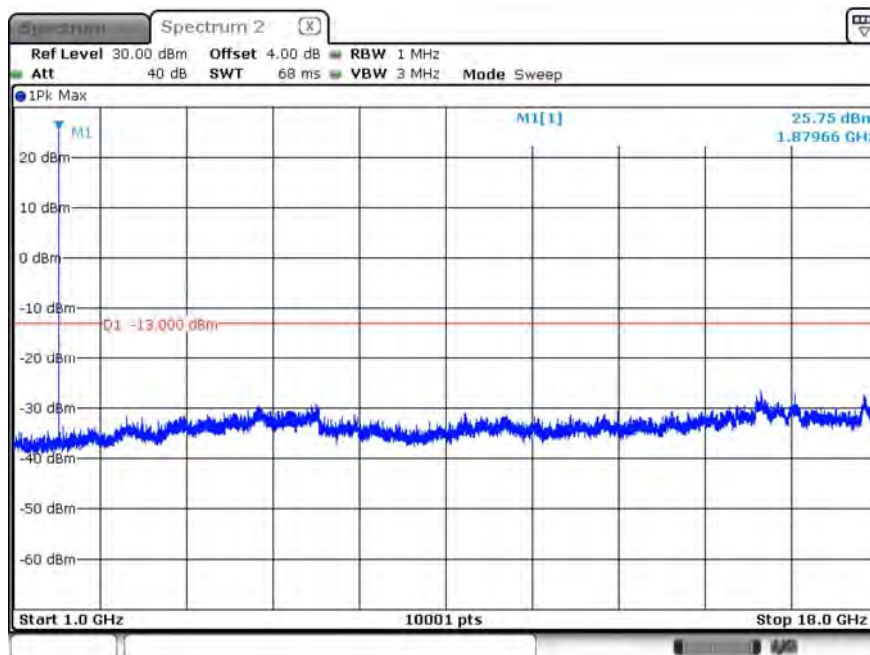
B2_CH18900_1.4M_1RB2_16-QAM_Above 1G
