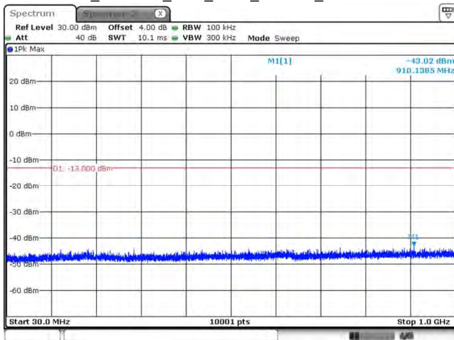
B2_CH18900_1.4M_1RB2_16-QAM_Below 1G
