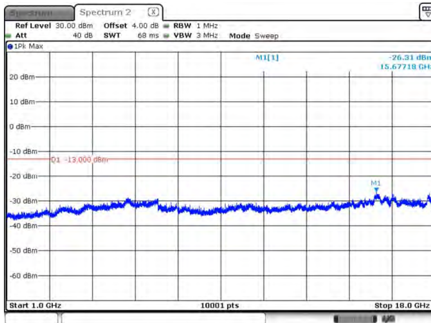
B12_CH23095_10M_1RB24_16-QAM_Above 1G
