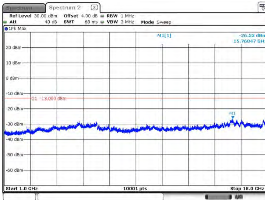
B26_CH26783_1.4M_1RB2_16-QAM_Above 1G
