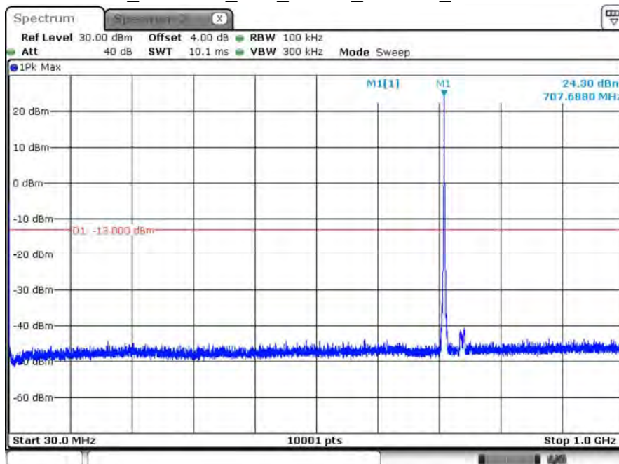
B12_CH23095_10M_1RB24_16-QAM_Below 1G
