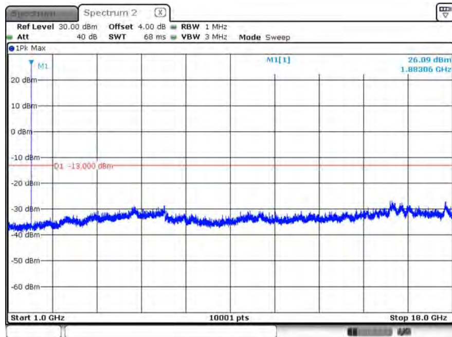
B25_CH26365_1.4M_1RB2_16-QAM_Above 1G
