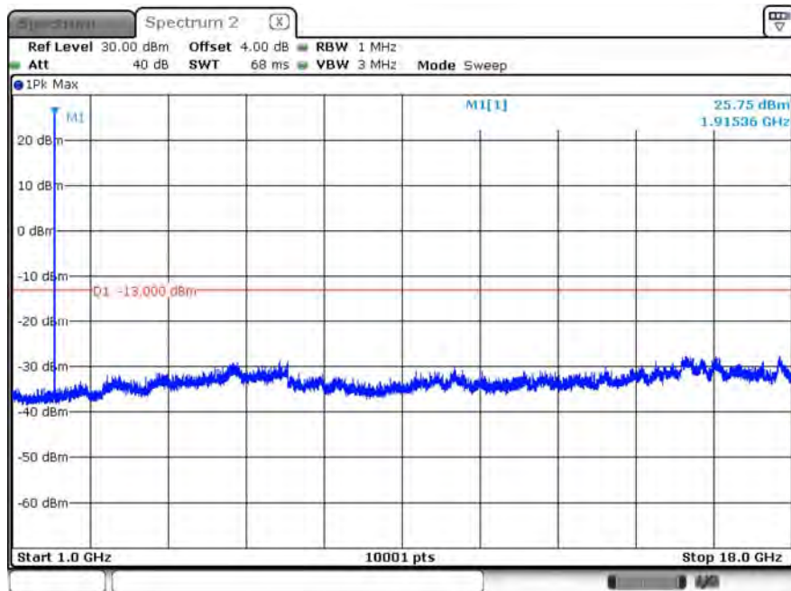
B25_CH26683_1.4M_1RB2_QPSK_Above 1G
