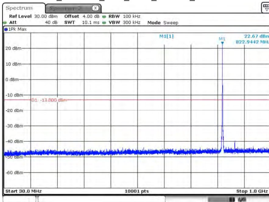
B26_CH26783_1.4M_1RB2_16-QAM_Below 1G
