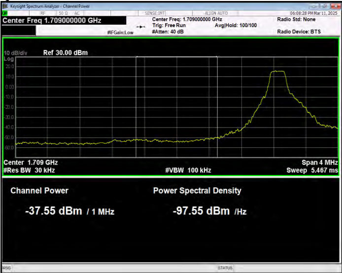
Band4 QPSK BW=1.4MHz Channel=19957 RB Size=#0 Extended
