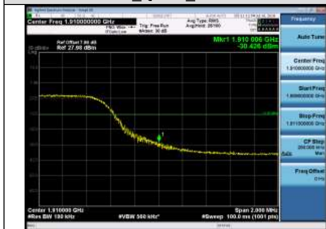
HCH_QPSK_50RB#0
