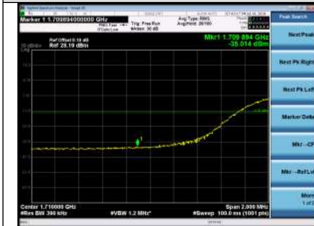
LCH_QPSK_100RB#0
