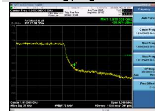
HCH_QPSK_6RB#0
