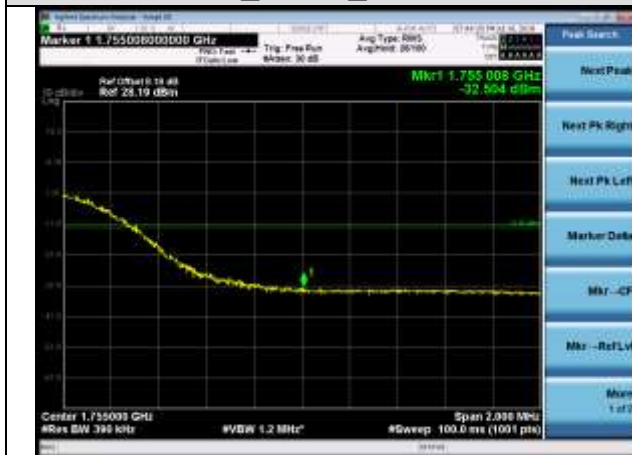
HCH_QPSK_100RB#0
