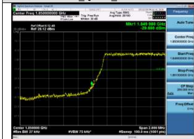
LCH_QPSK_6RB#0
