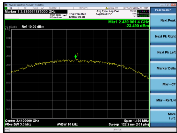
Bluetooth Low Energy 1Mbps 2440MHz
