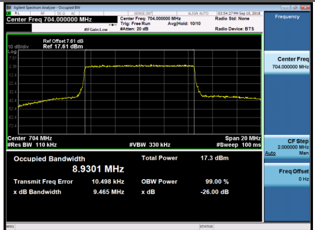
LCH_16QAM_50RB#0
