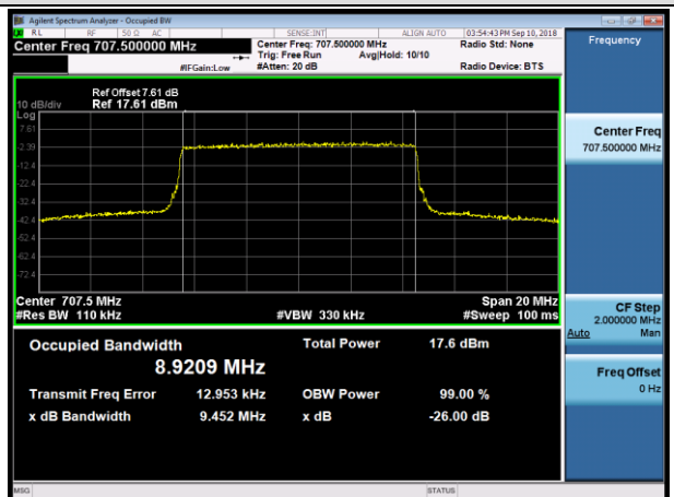
MCH_16QAM_50RB#0
