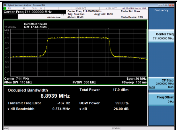
HCH_16QAM_50RB#0
