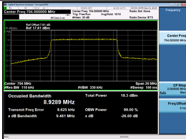
LCH_QPSK_50RB#0
