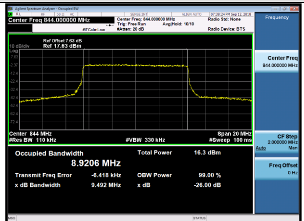
HCH_16QAM_50RB#0
