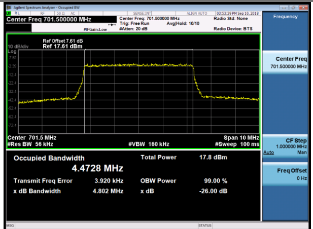
LCH_16QAM_25RB#0
