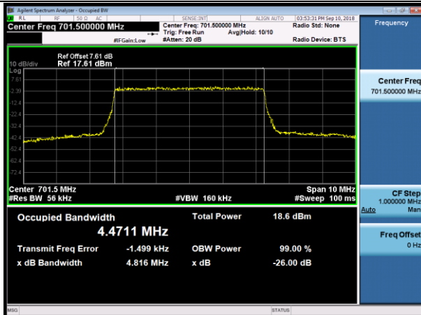
LCH_QPSK_25RB#0
