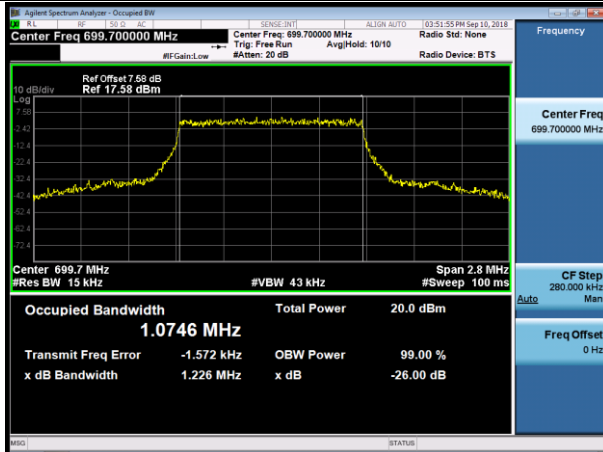
LCH_QPSK_6RB#0
