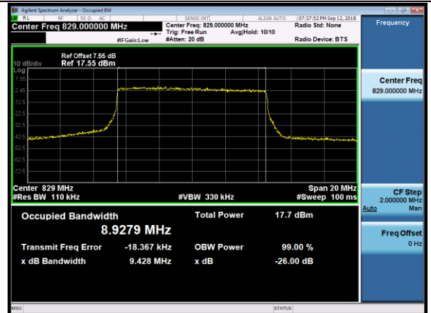
LCH_16QAM_50RB#0
