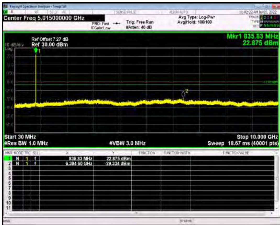
HSUPA Band5 Subtest1 Channel=4233 Band5 Normal
