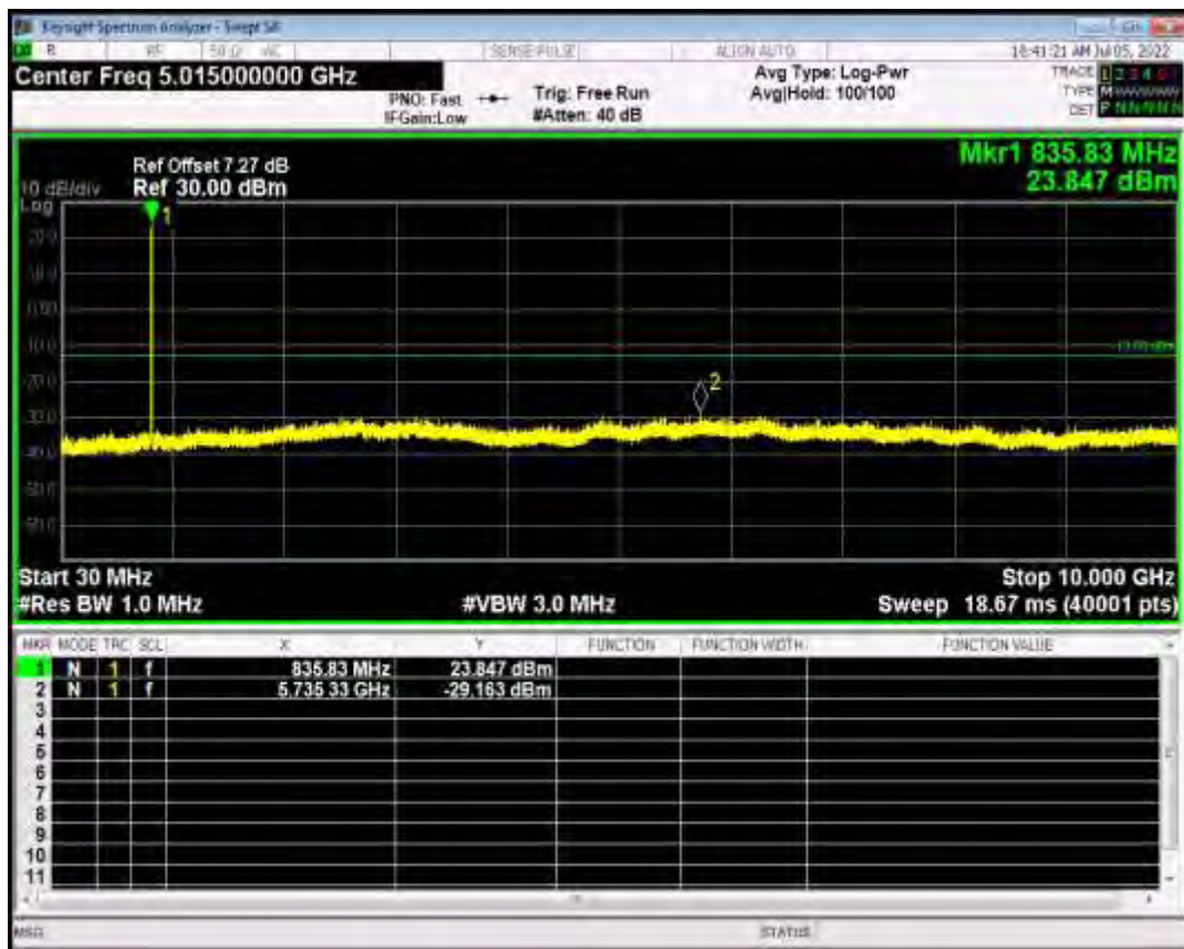
WCDMA Band5 Channel=4233 Band5 Normal
