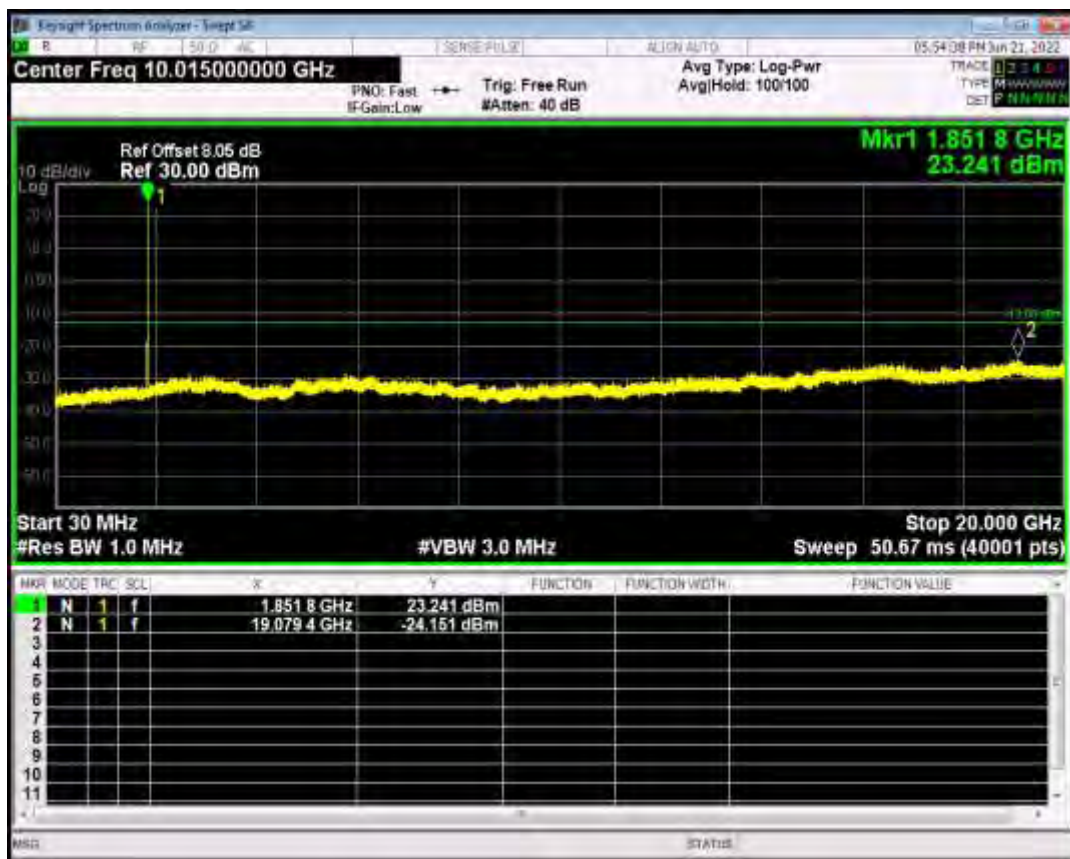
HSDPA Band2 Subtest1 Channel=9400 Band2 Normal
