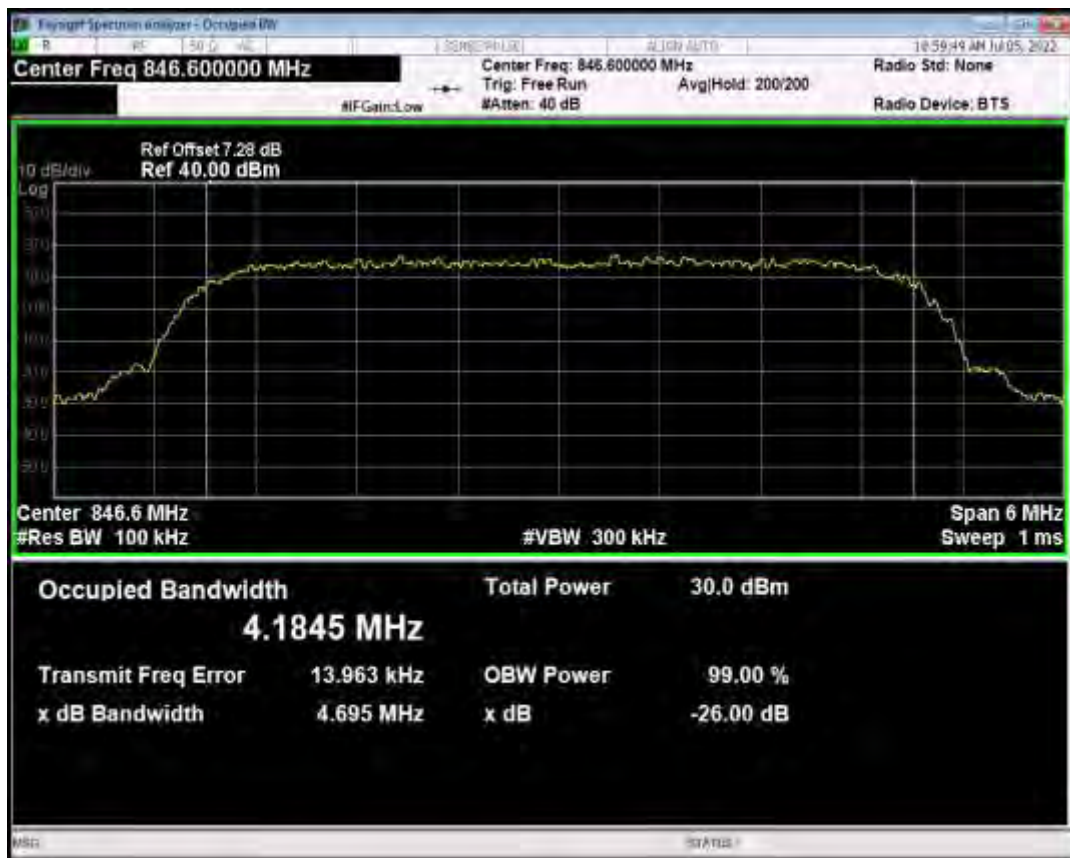
WCDMA Band2 Channel=9262 Band2 Normal
