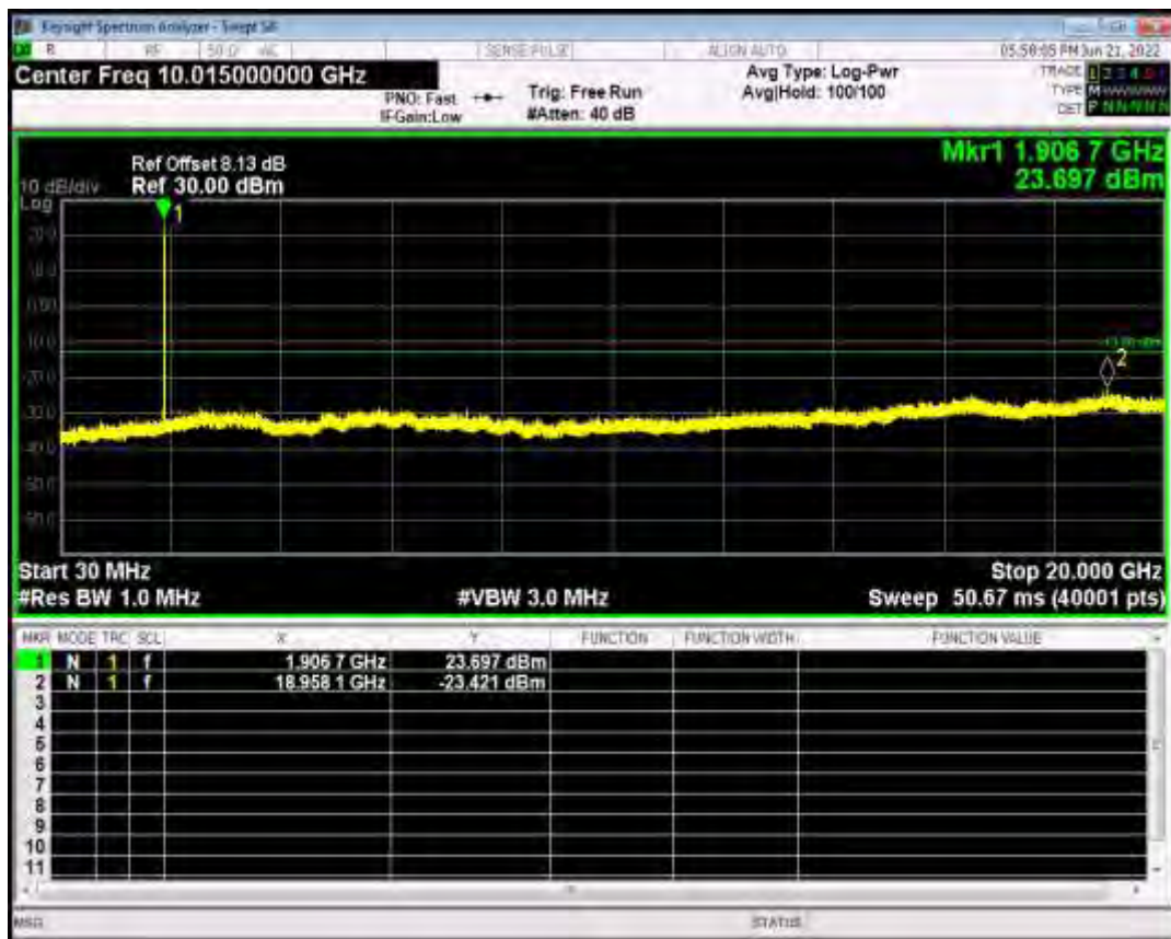
HSDPA Band2 Subtest2 Channel=9262 Band2 Normal
