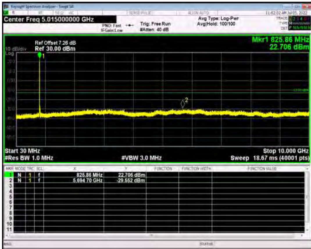
HSUPA Band5 Subtest5 Channel=4182 Band5 Normal
