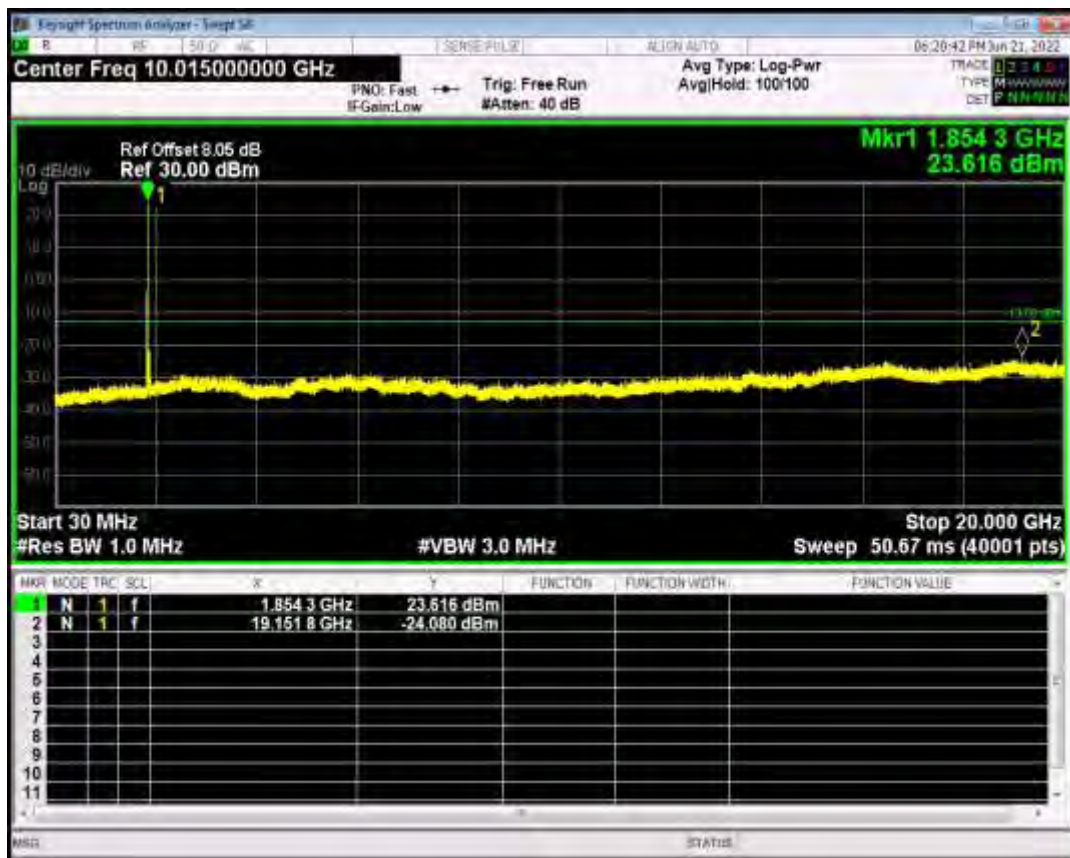
HSUPA Band2 Subtest3 Channel=9400 Band2 Normal
