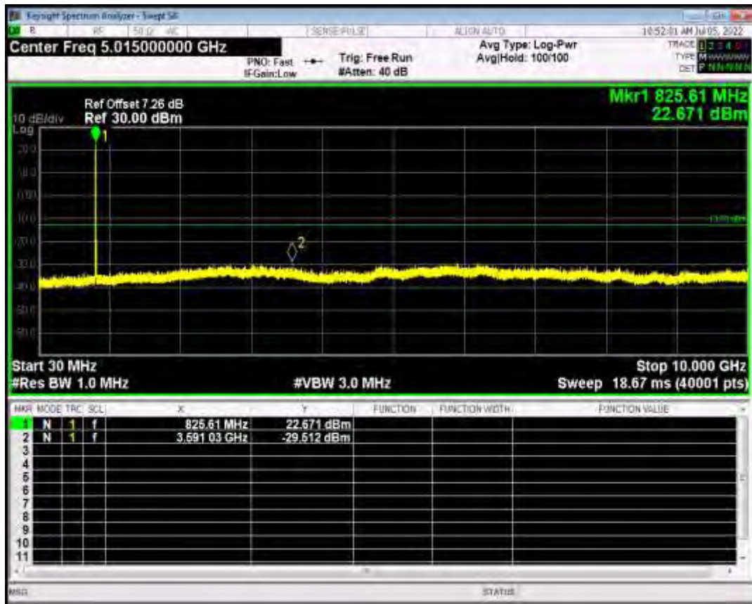
HSDPA Band5 Subtest4 Channel=4182 Band5 Normal
