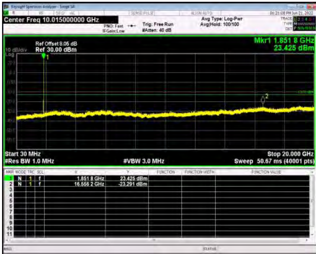
HSUPA Band2 Subtest4 Channel=9400 Band2 Normal
