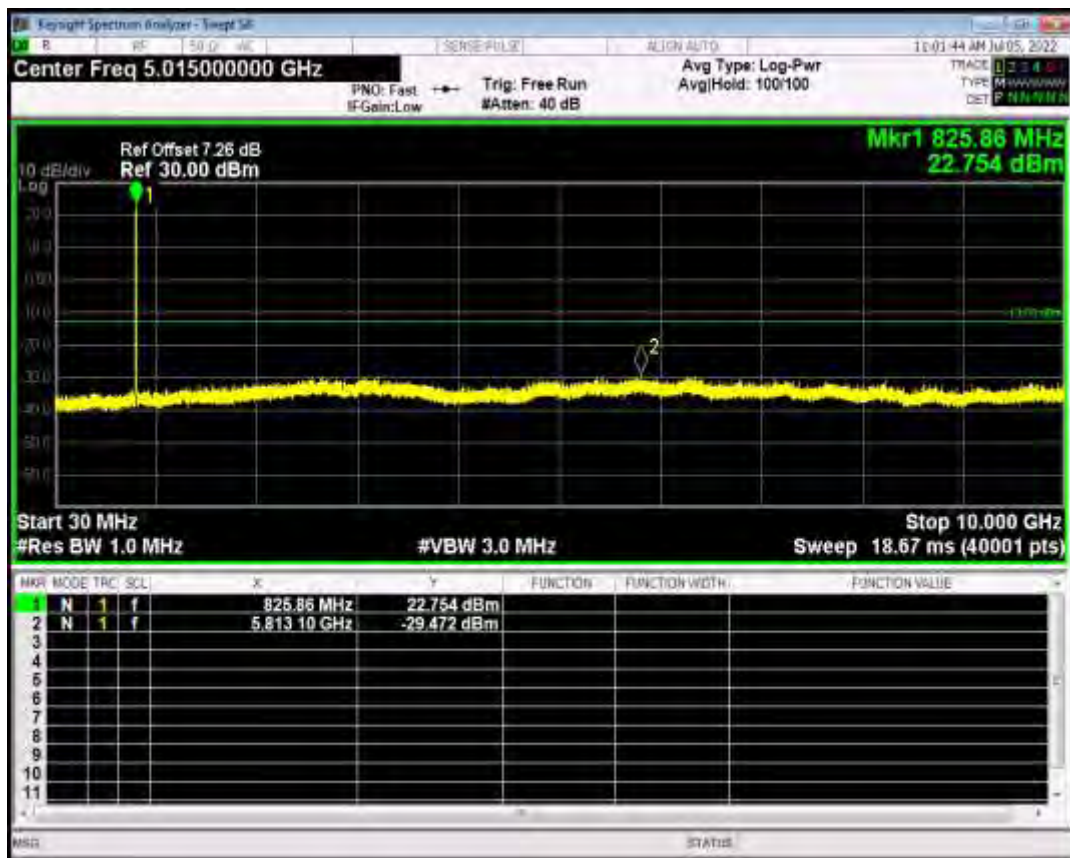
HSUPA Band5 Subtest4 Channel=4182 Band5 Normal
