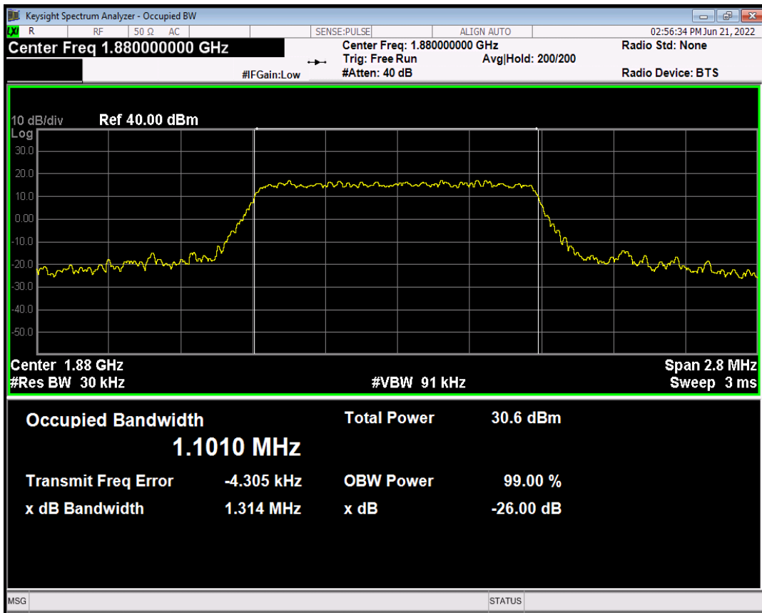
Band2 QAM16 BW=10MHz Channel=18900 RB Size=50 Position=#0 Band2 Normal
