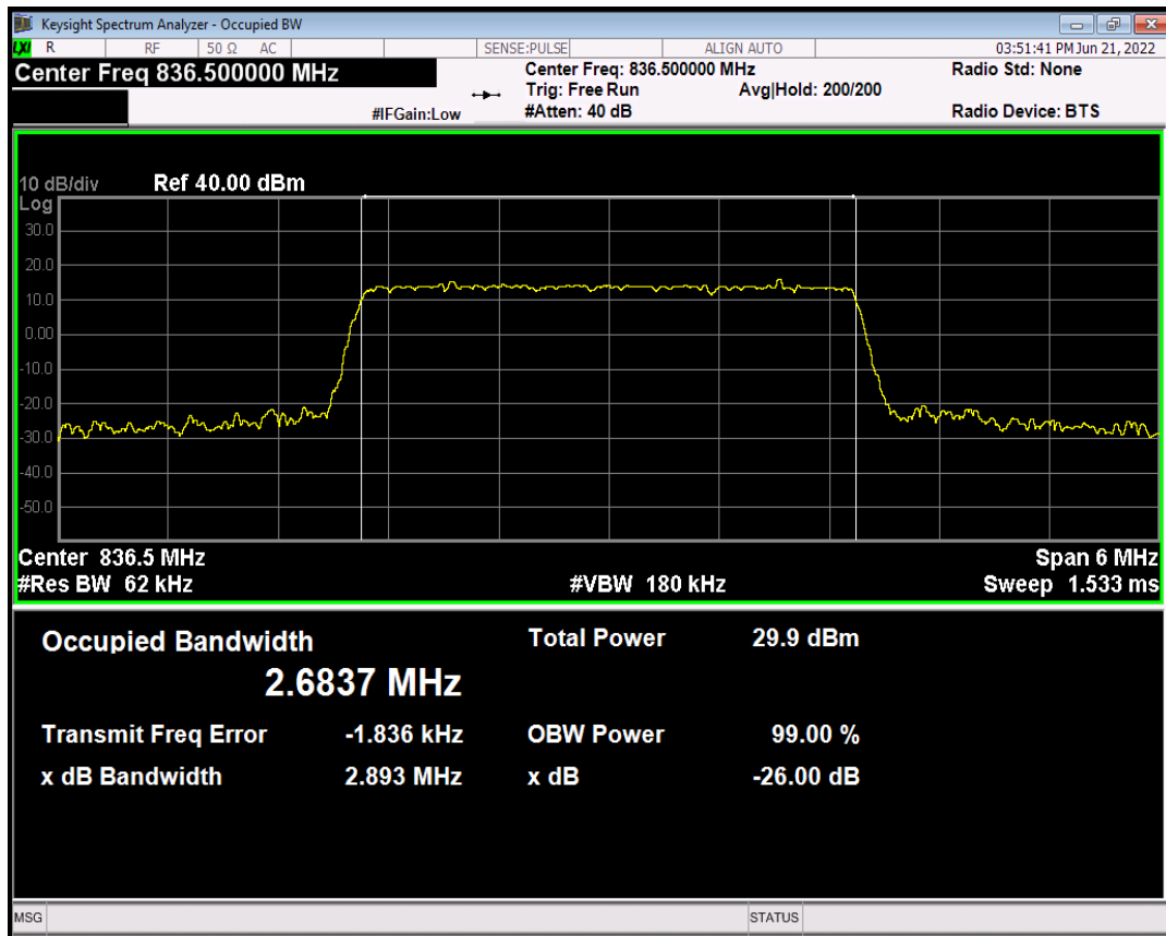
Band5 QAM16 BW=5MHz Channel=20525 RB Size=25 Position=#0 Band5 Normal
