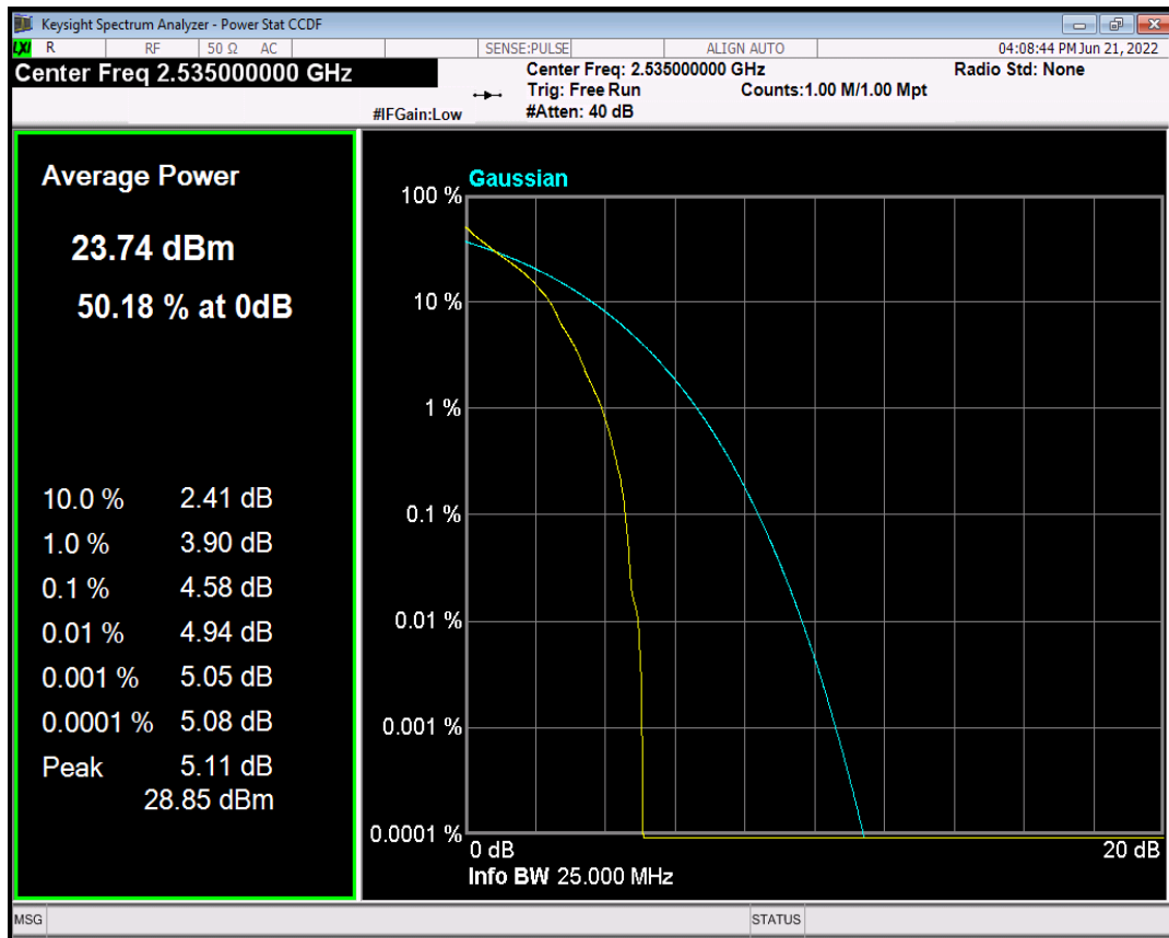
Band7 QPSK BW=20MHz Channel=21100 RB Size=1 Position=#0 Band7 Normal
