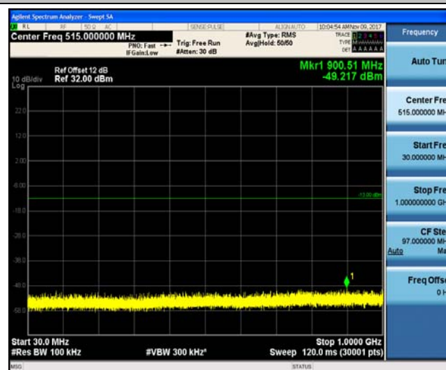
Band4 3MHz 16QAM 19965 1RB#0
