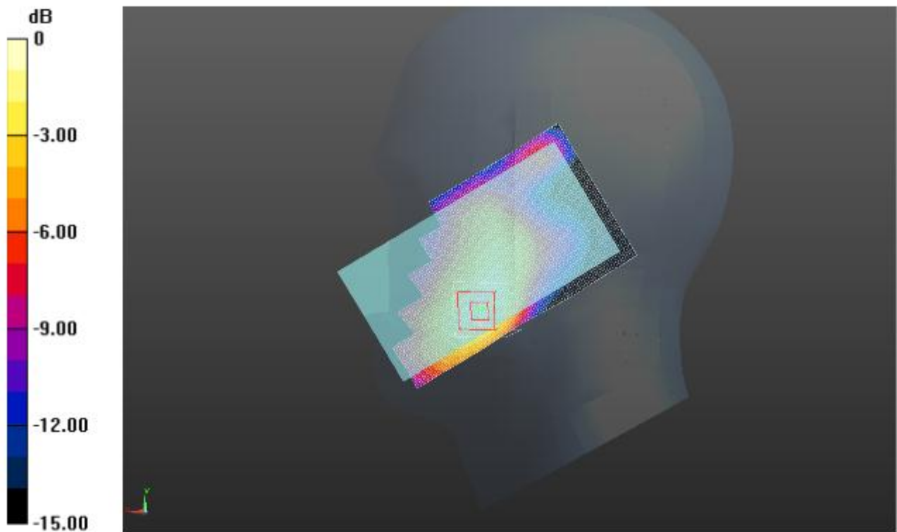
Left Head Cheek (LTE Band 4 Middle Channel)
