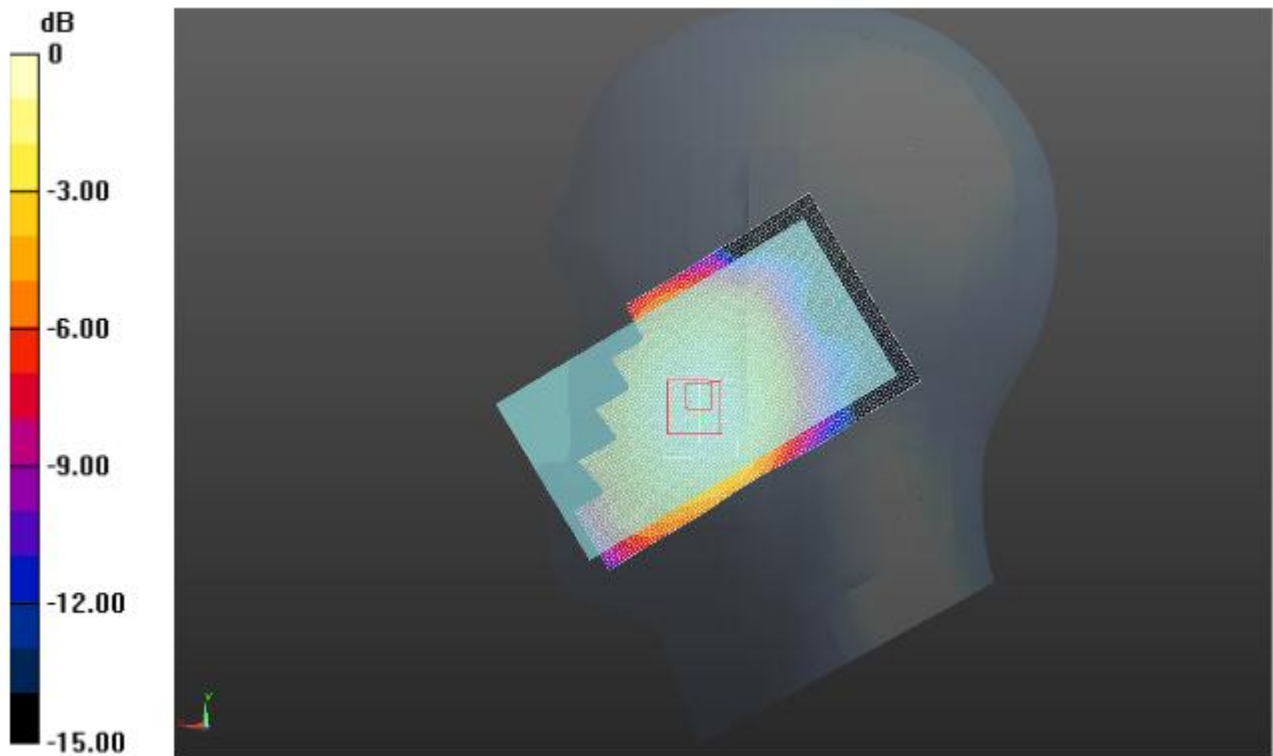
Left Head Cheek (LTE Band 12 Middle Channel)
