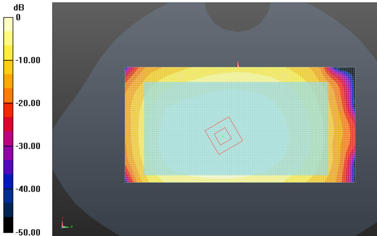
Body- worn Rear Side (LTE Band 17 Middle Channel)
