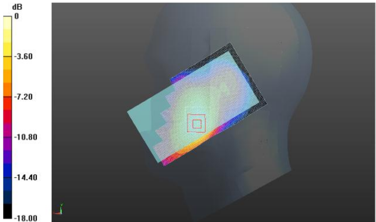
Left Head Cheek (LTE Band 2 Middle Channel)
