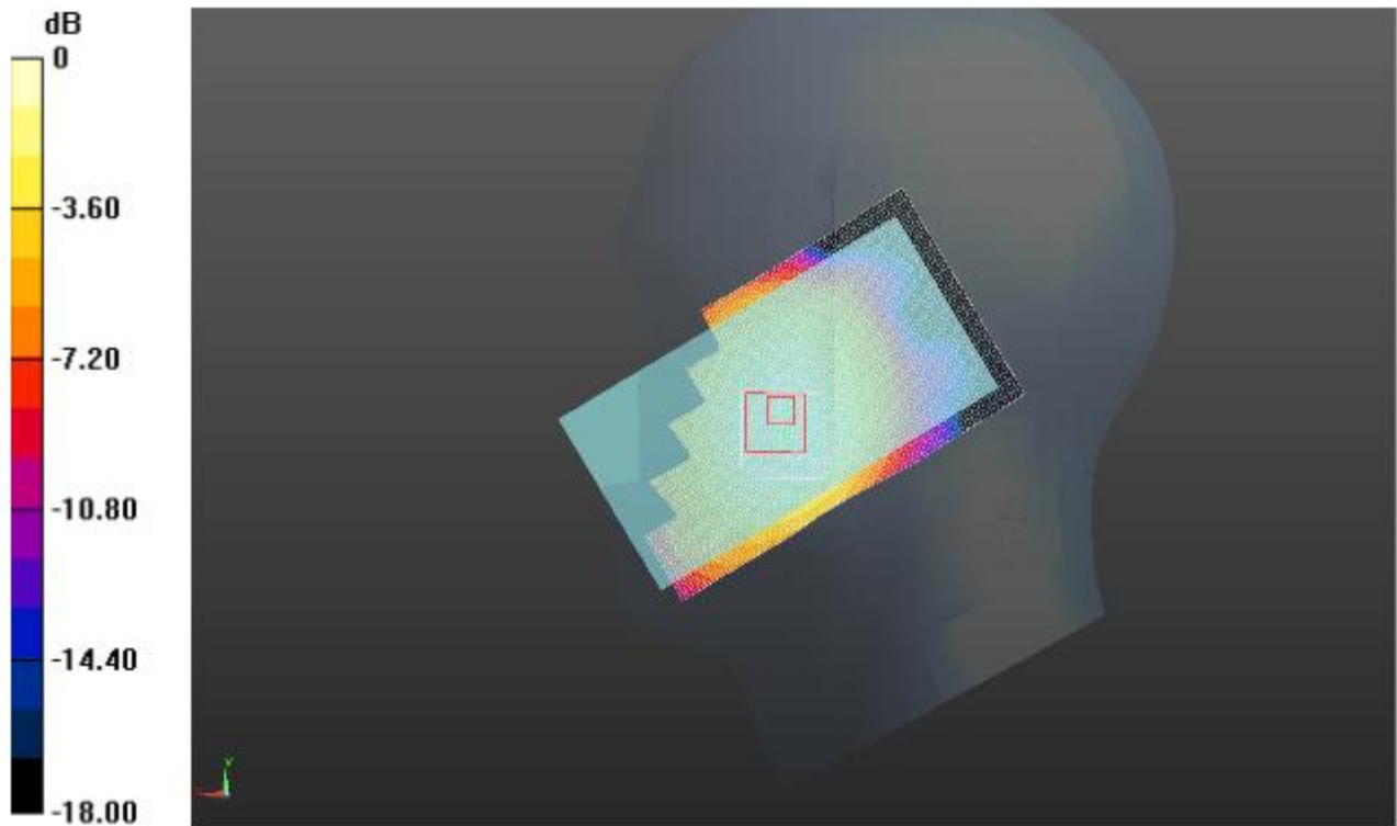
Left Head Cheek (LTE Band 17 Middle Channel)
