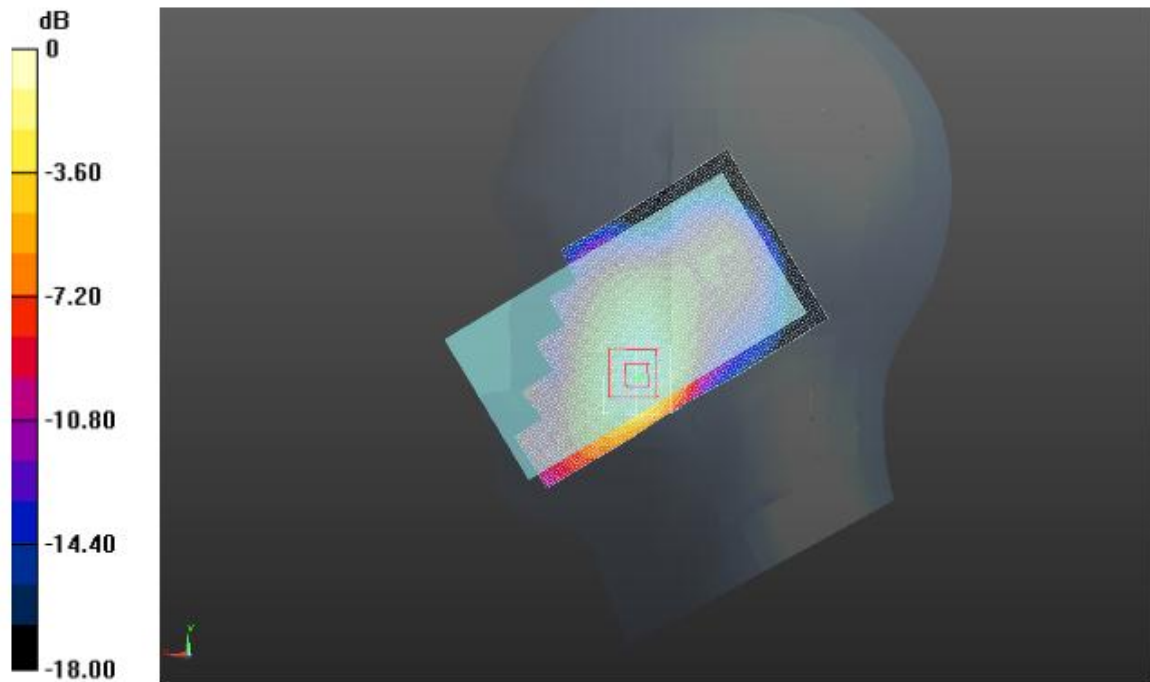
Left Head Cheek (PCS1900 GPRS 4TS Middle Channel)
