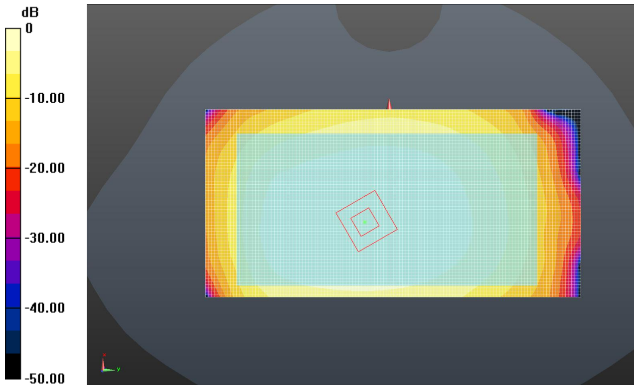
Body- worn Rear Side (LTE Band 12 Middle Channel)
