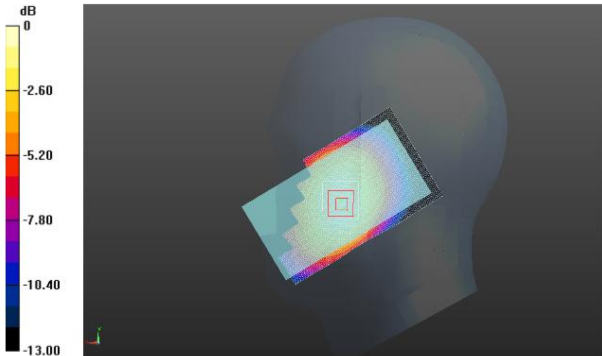
Left Head Cheek (LTE Band 5 Middle Channel)
