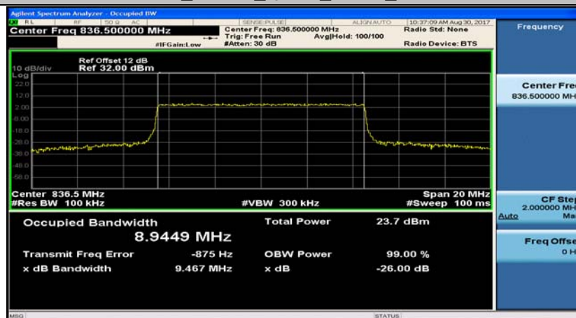
Band5_10MHz_16QAM_20525_50RB#0
