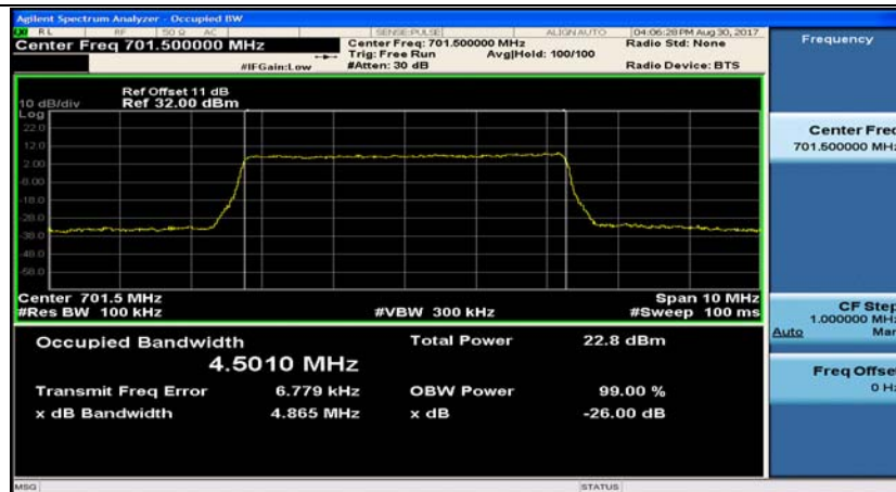
Band12_5MHz_16QAM_23035_25RB#0
