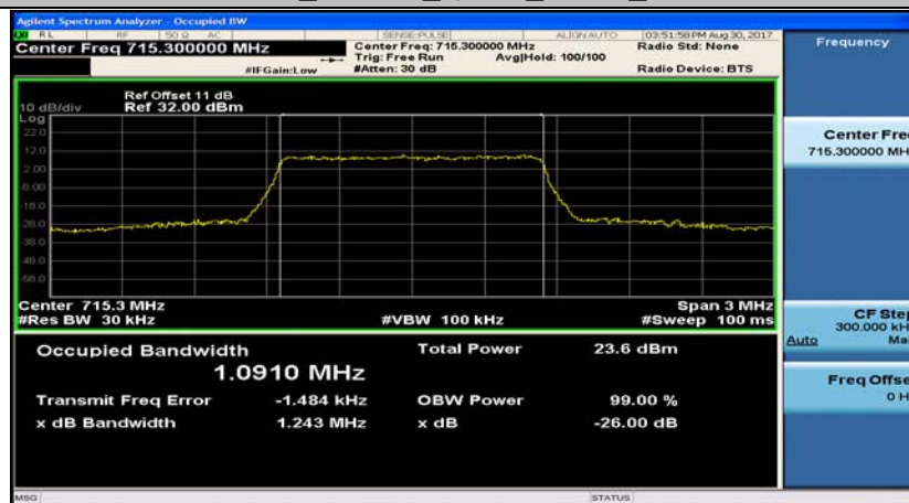
Band12_1.4MHz_16QAM_23173_6RB#0
