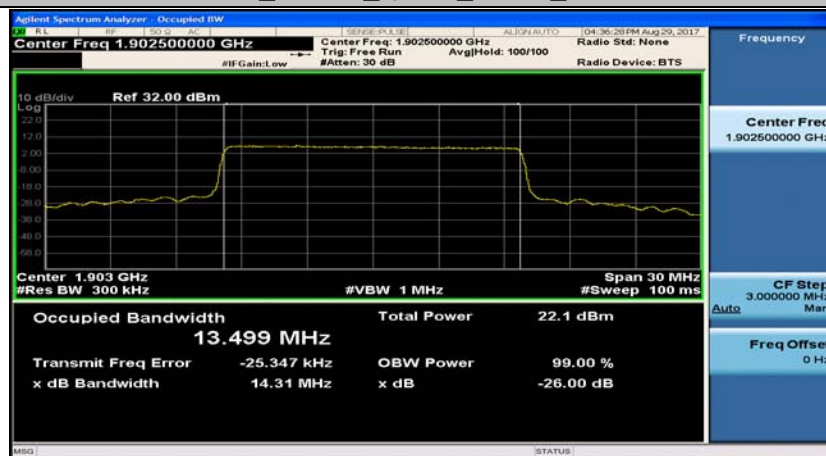
Band2_15MHz_16QAM_19125_75RB#0
