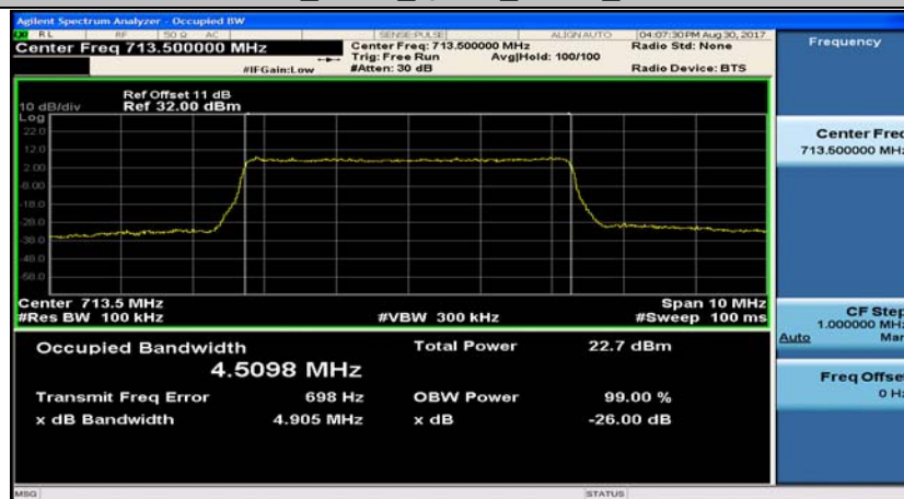
Band12_5MHz_16QAM_23155_25RB#0
