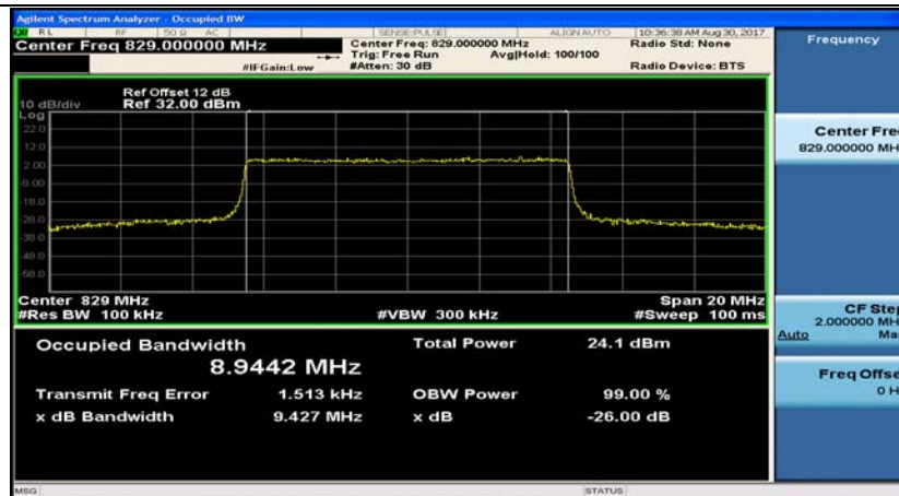
Band5_10MHz_16QAM_20450_50RB#0
