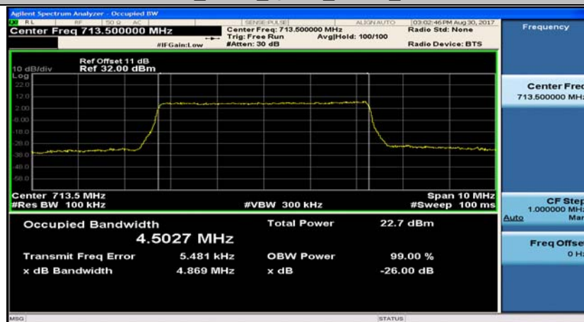
Band17_5MHz_16QAM_23825_25RB#0
