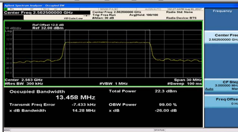
Band7_15MHz_16QAM_21375_75RB#0
