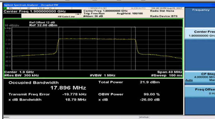
Band2_20MHz_16QAM_19100_100RB#0
