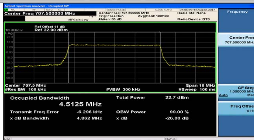
Band12_5MHz_16QAM_23095_25RB#0
