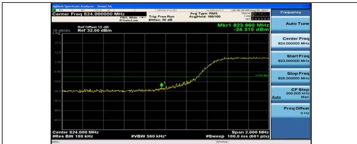
Band5_10MHz_QPSK_20600_50RB#0
