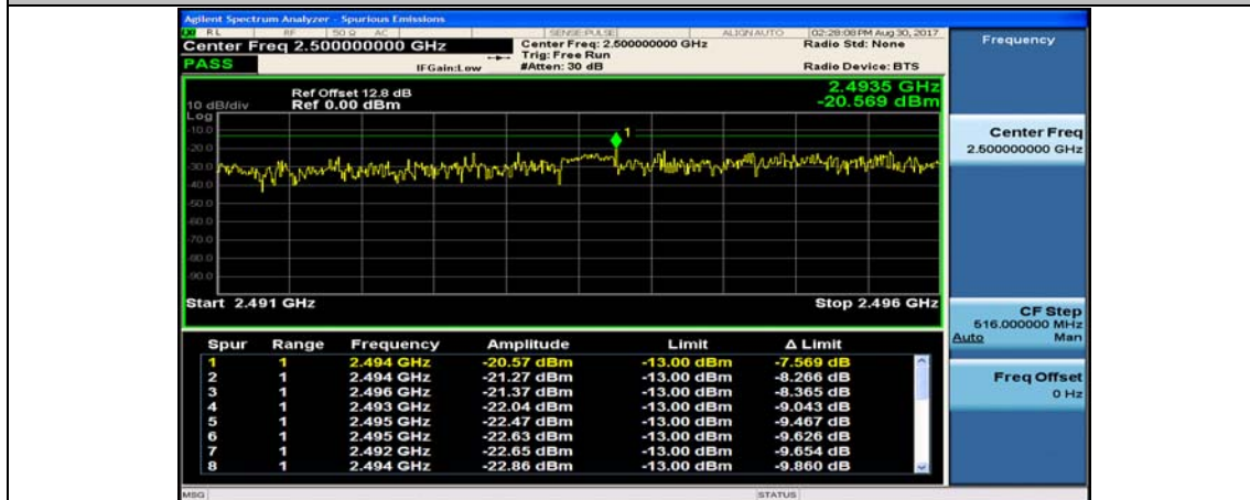
Band7_15MHz_16QAM_20825_75RB#0
