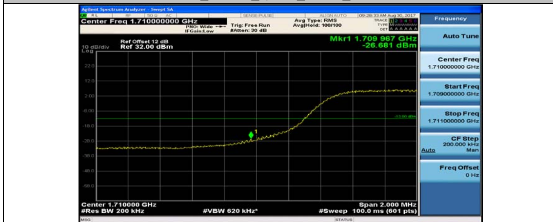
Band4_10MHz_16QAM_20000_50RB#0
