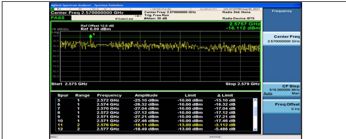
Band7_10MHz_16QAM_21400_50RB#0
