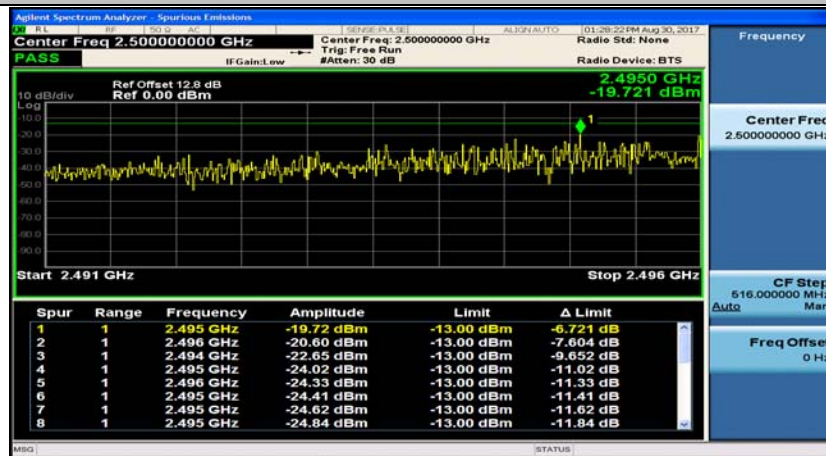
Band7_5MHz_QPSK_21425_25RB#0
