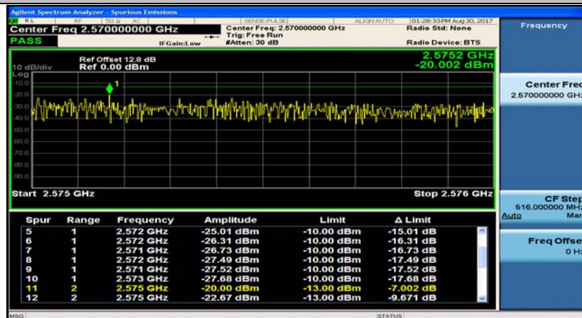
Band7_5MHz_16QAM_21425_25RB#0
