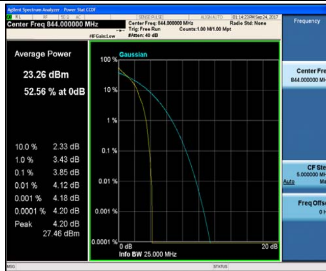
Band5_10MHz_16QAM_20600_1RB#0_4.97_13_PASS
