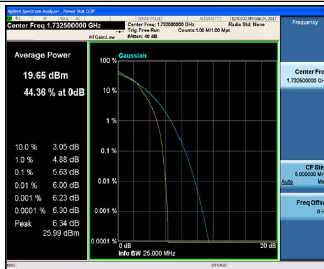
Band4_15MHz_QPSK_20325_1RB#0_3.19_13_PASS
