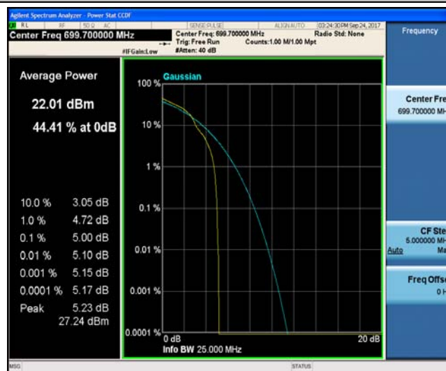
Band12_1.4MHz_QPSK_23017_6RB#0_5.06_13_PASS
