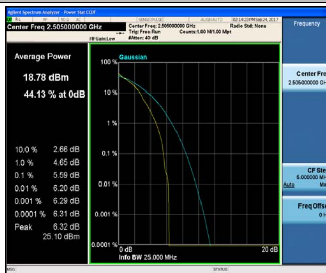
Band7_10MHz_16QAM_20800_1RB#0_6.29_13_PASS
