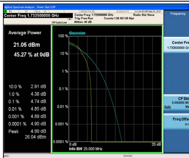
Band4_20MHz_QPSK_20300_100RB#0_4.97_13_PASS
