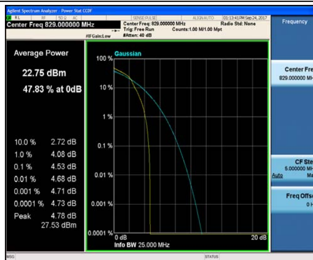
Band5_10MHz_QPSK_20450_50RB#0_4.90_13_PASS
