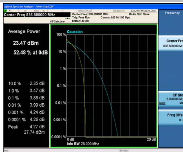
Band5_3MHz_16QAM_20525_1RB#0_4.80_13_PASS
