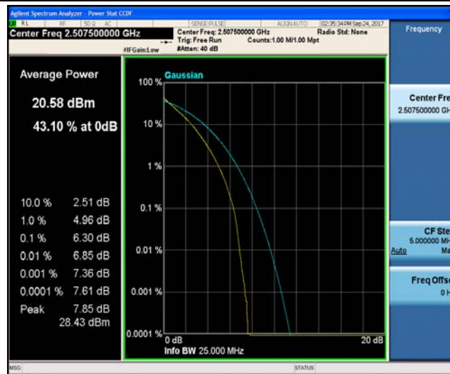
Band7_15MHz_16QAM_20825_75RB#0_6.80_13_PASS
