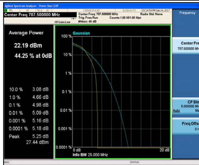
Band12_1.4MHz_QPSK_23095_6RB#0_4.98_13_PASS
