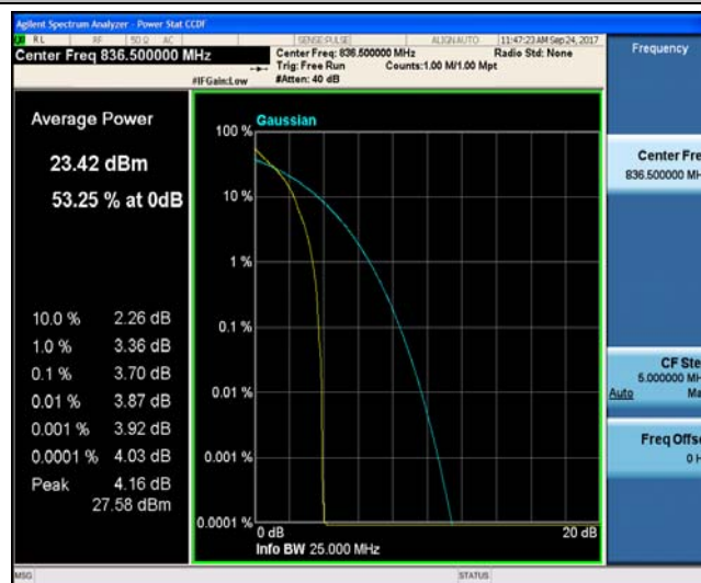
Band5_1.4MHz_16QAM_20525_1RB#0_4.63_13_PASS
