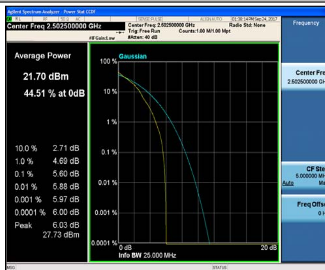
Band7_5MHz_16QAM_20775_1RB#0_6.80_13_PASS
