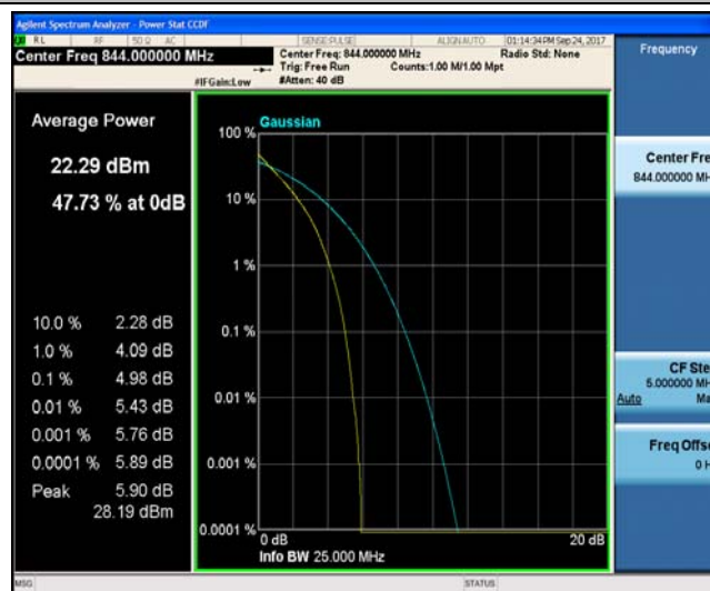
Band5_10MHz_16QAM_20600_50RB#0_5.79_13_PASS
