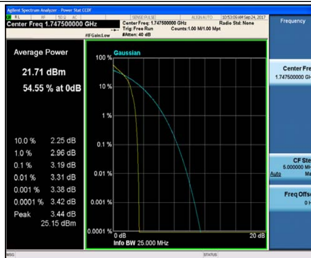
Band4_15MHz_16QAM_20325_1RB#0_4.21_13_PASS
