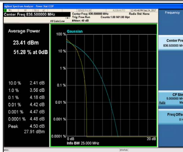
Band5_5MHz_16QAM_20525_1RB#0_4.82_13_PASS
