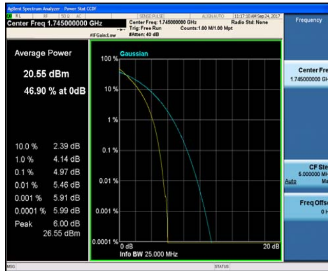
Band4_20MHz_16QAM_20300_100RB#0_5.81_13_PASS
