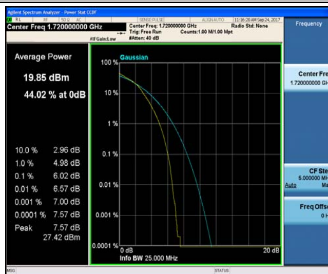
Band4_20MHz_QPSK_20050_1RB#0_3.21_13_PASS
