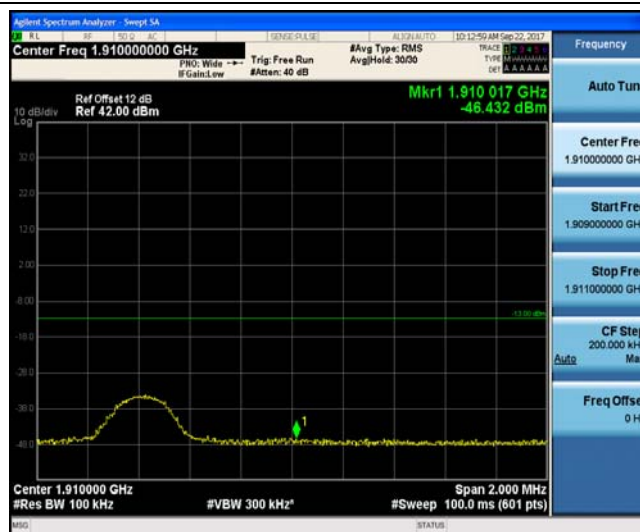
Band2_10MHz_16QAM_19150_1RB#0_-46.00_PASS
