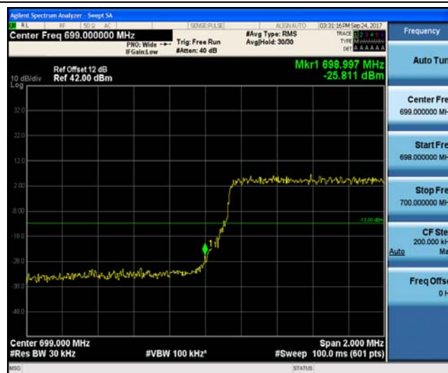
Band12_3MHz_QPSK_23025_1RB#0_-14.60_PASS
