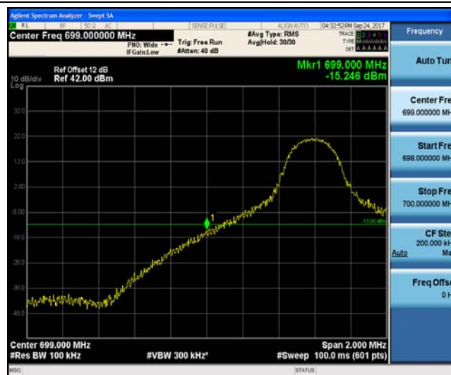
Band12_10MHz_QPSK_23060_50RB#0_-28.81_PASS
