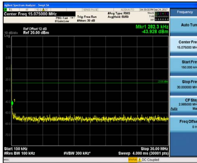
Band12_10MHz_16QAM_23095_1RB#0_Range3:30~1000MHz_-38.64_PASS
