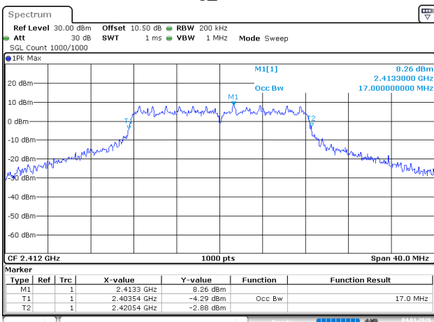
802.11g_2412MHz
